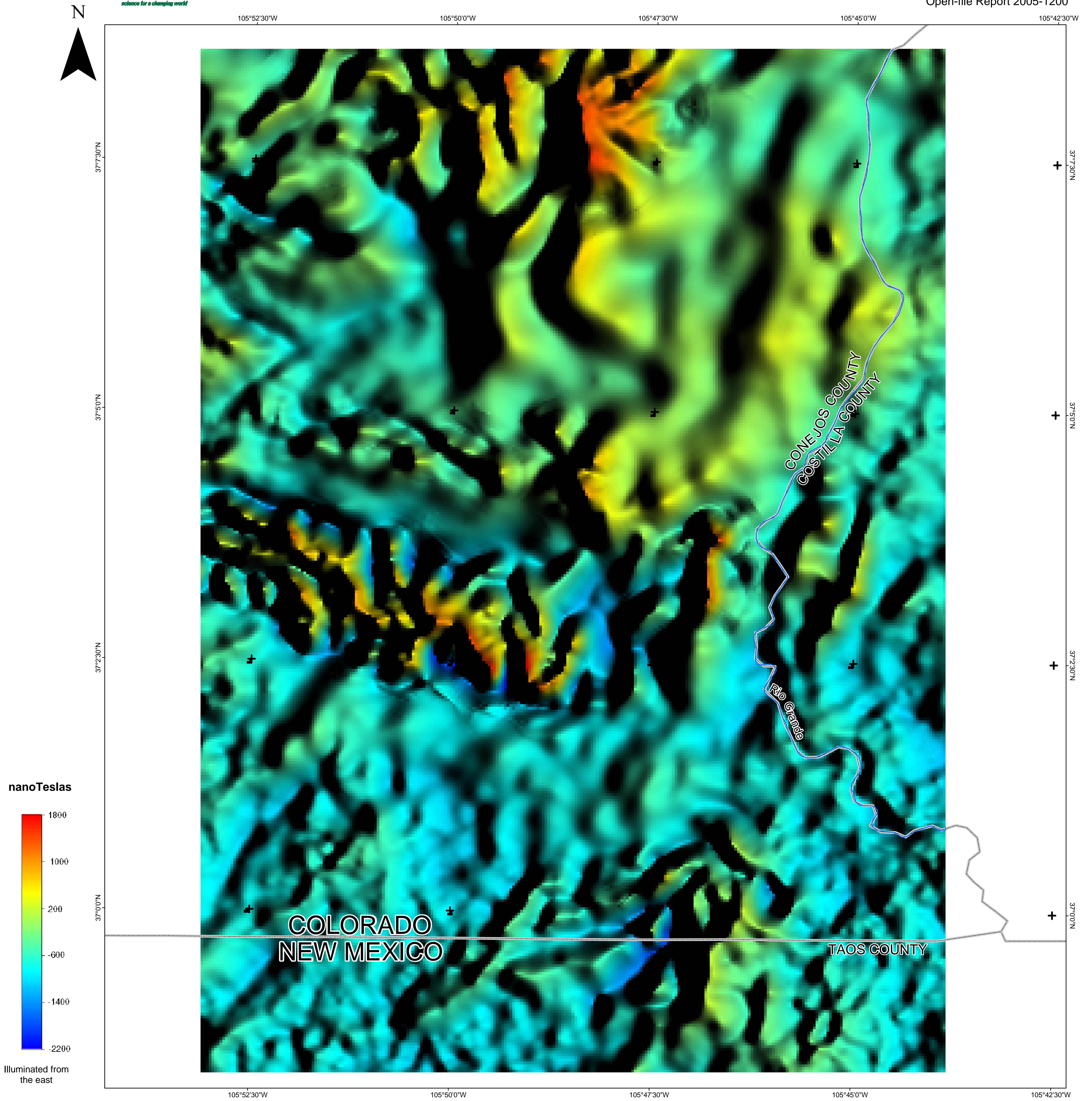
Central San Luis Basin Aeromagnetic Survey Color shaded-relief image of continued, reduced-to-pole (RTP) magnetic data, Kiowa Hill area.
