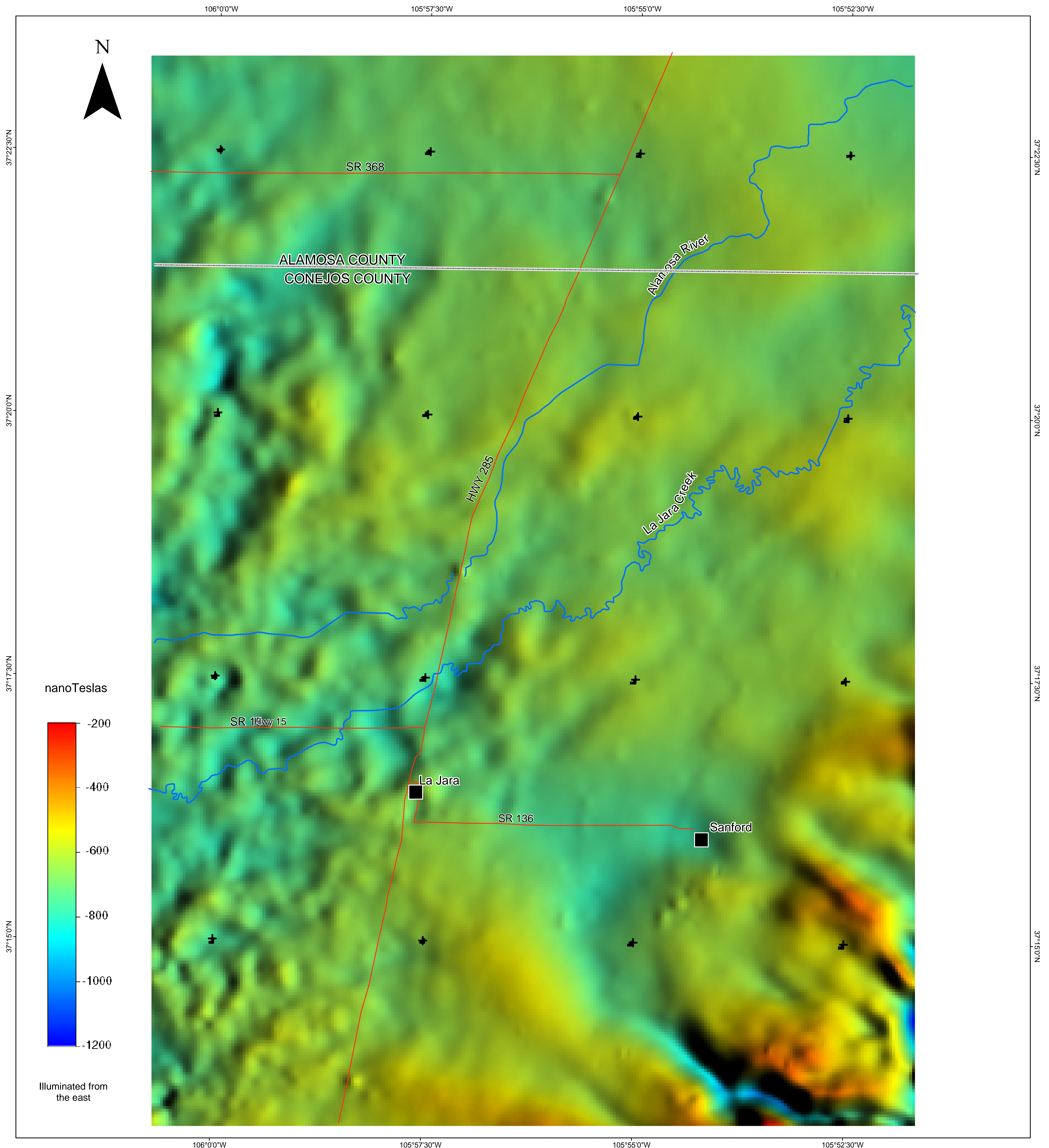
Central San Luis Basin Aeromagnetic Survey Color shaded-relief image of continued, reduced-to-pole (RTP) magnetic data, La Jara area.
