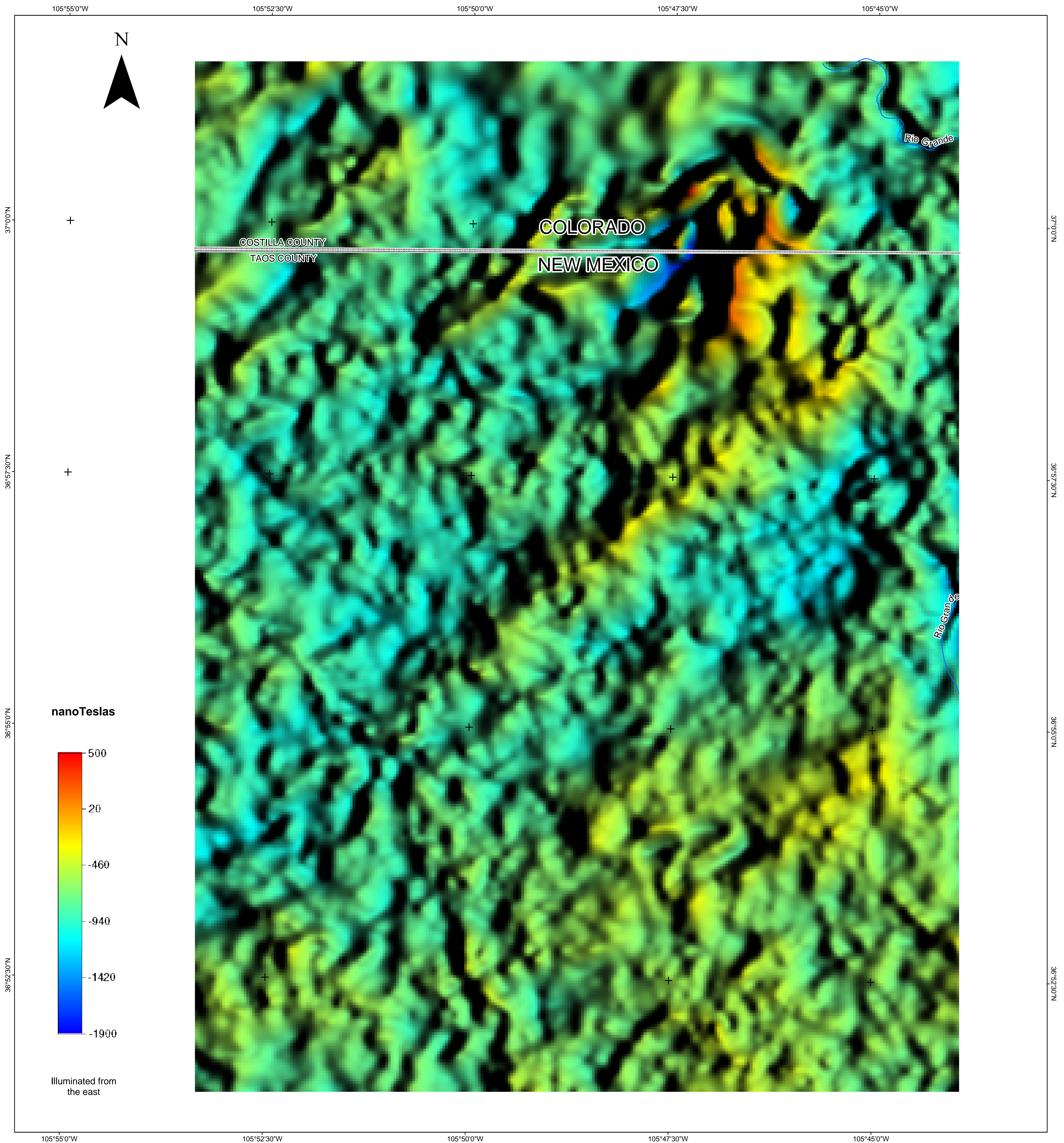
Central San Luis Basin Aeromagnetic Survey Color shaded-relief image of continued, reduced-to-pole (RTP) magnetic data, La Segita Peaks NE area.
