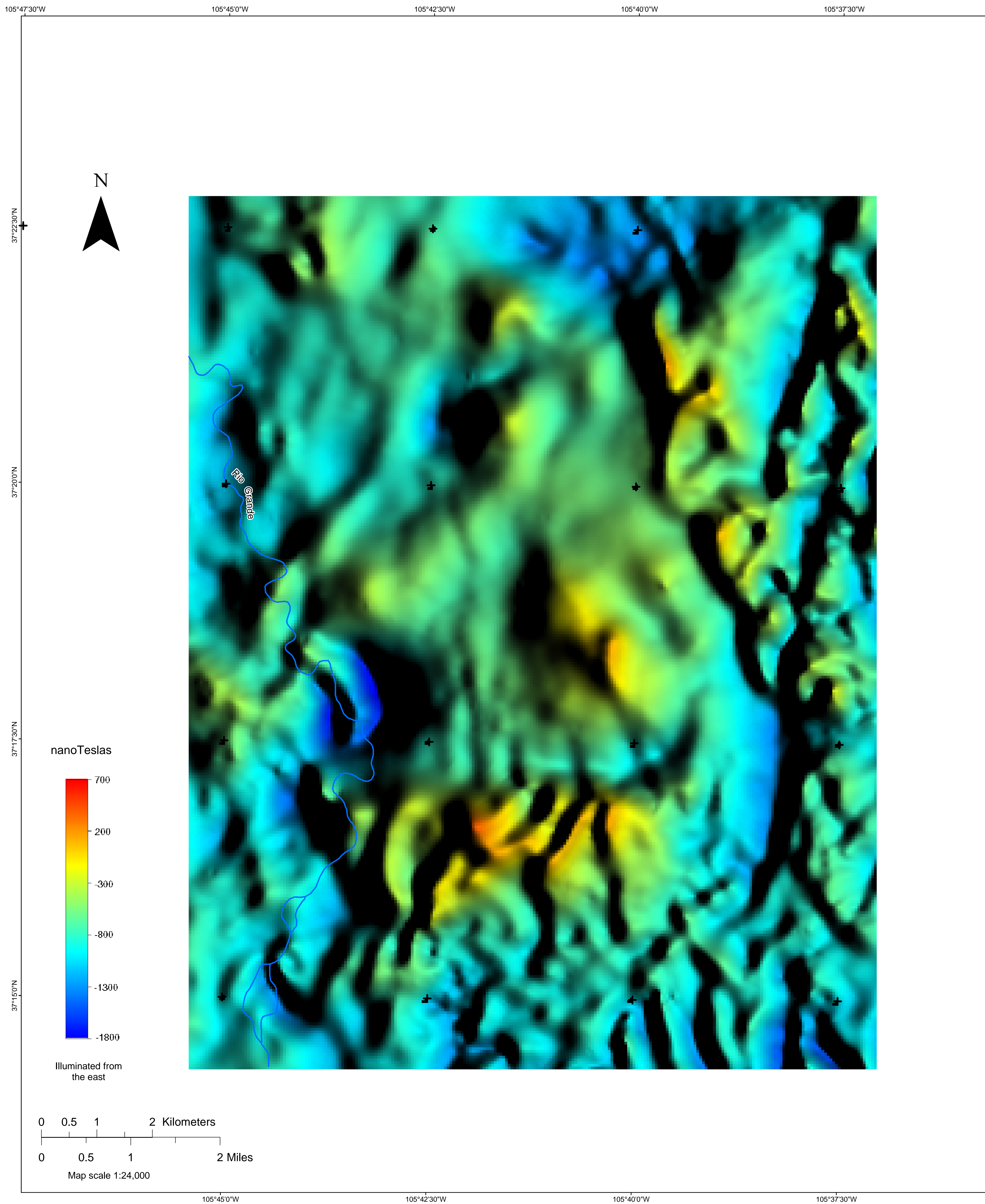
Central San Luis Basin Aeromagnetic Survey Color shaded-relief image of continued, reduced-to-pole (RTP) magnetic data, La Sauses area.
