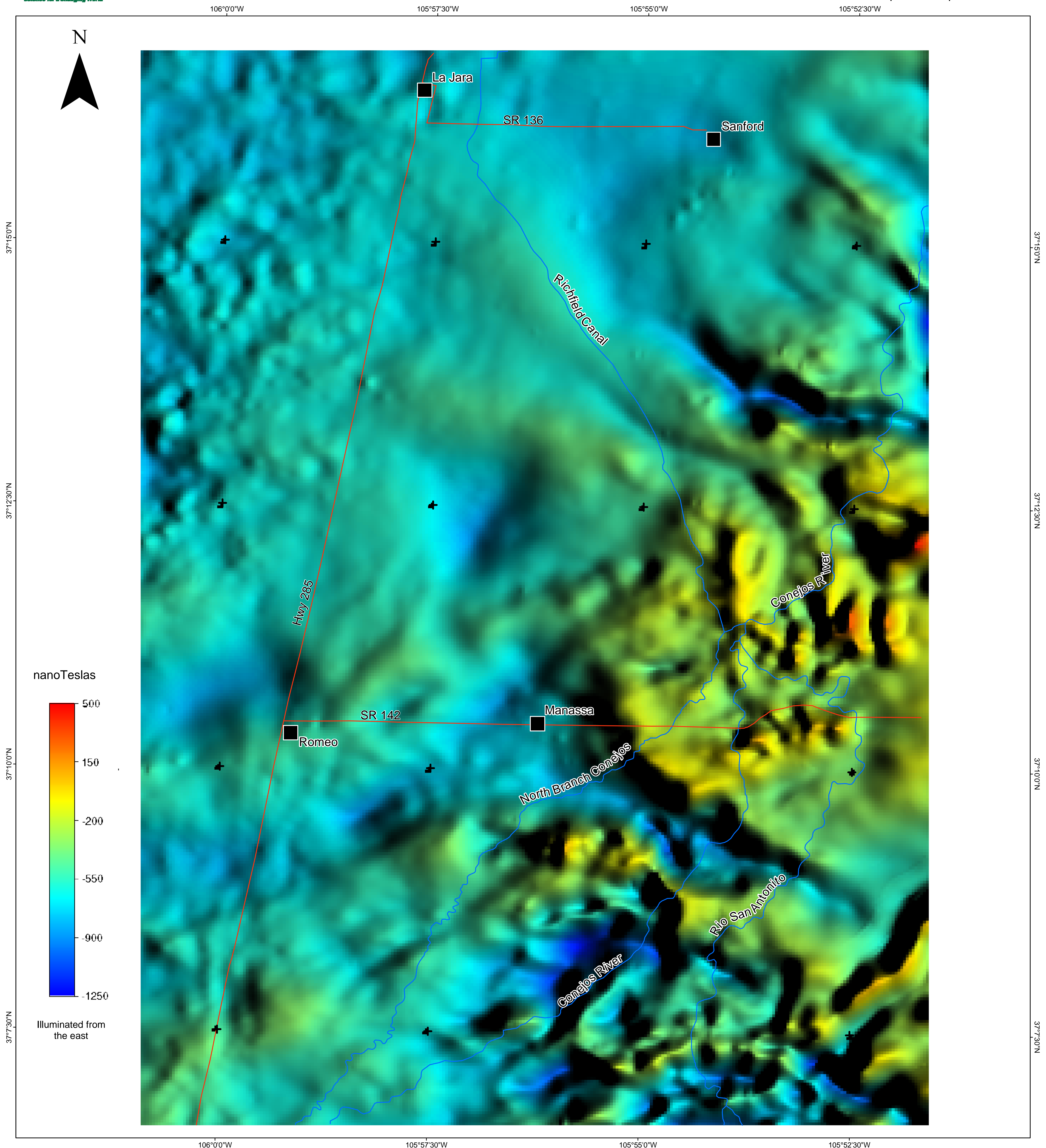
Central San Luis Basin Aeromagnetic Survey Color shaded-relief image of continued, reduced-to-pole (RTP) magnetic data, Manassa area.
