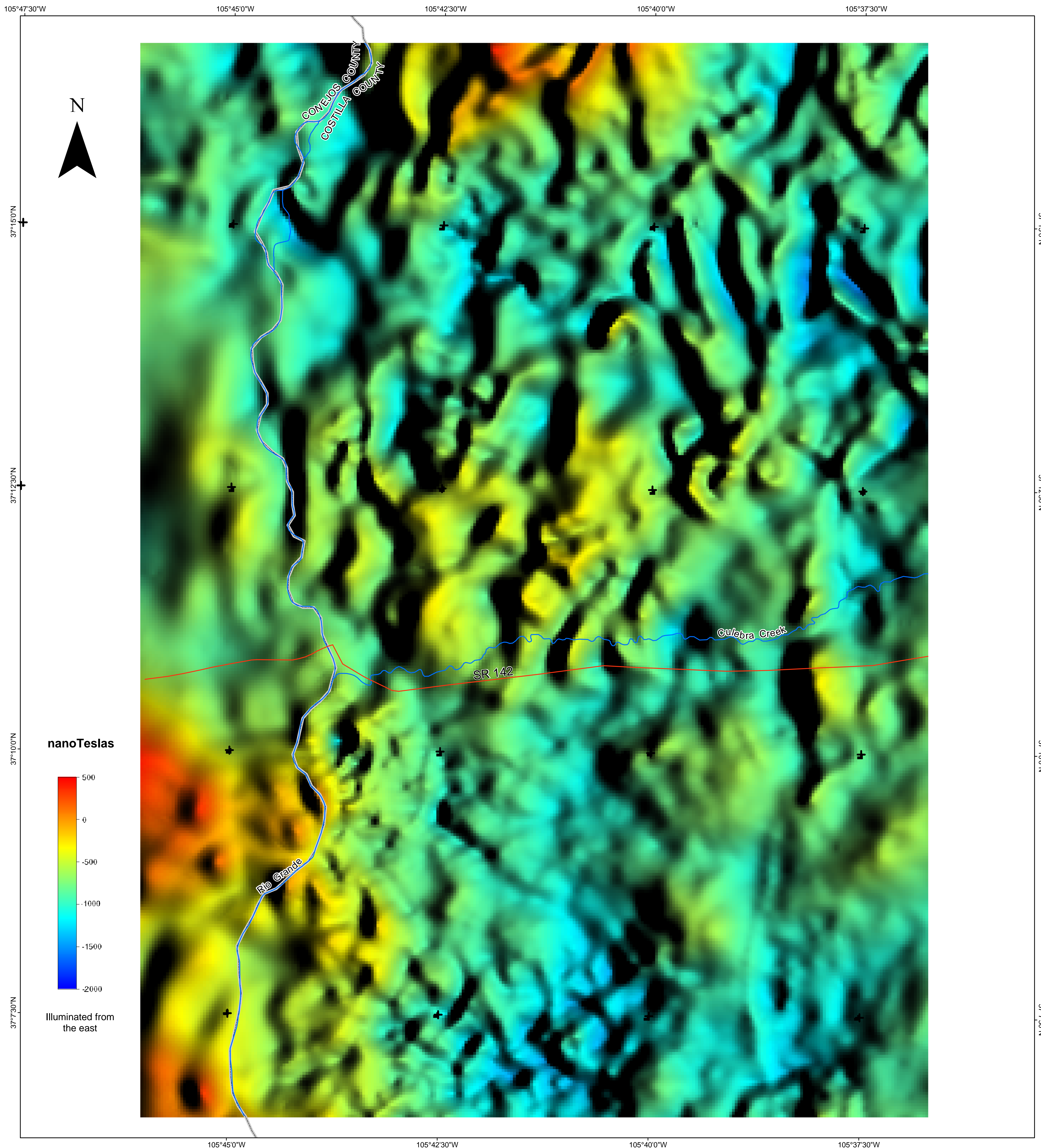
Central San Luis Basin Aeromagnetic Survey Color shaded-relief image of continued, reduced-to-pole (RTP) magnetic data, Mesito Reservoir area.
