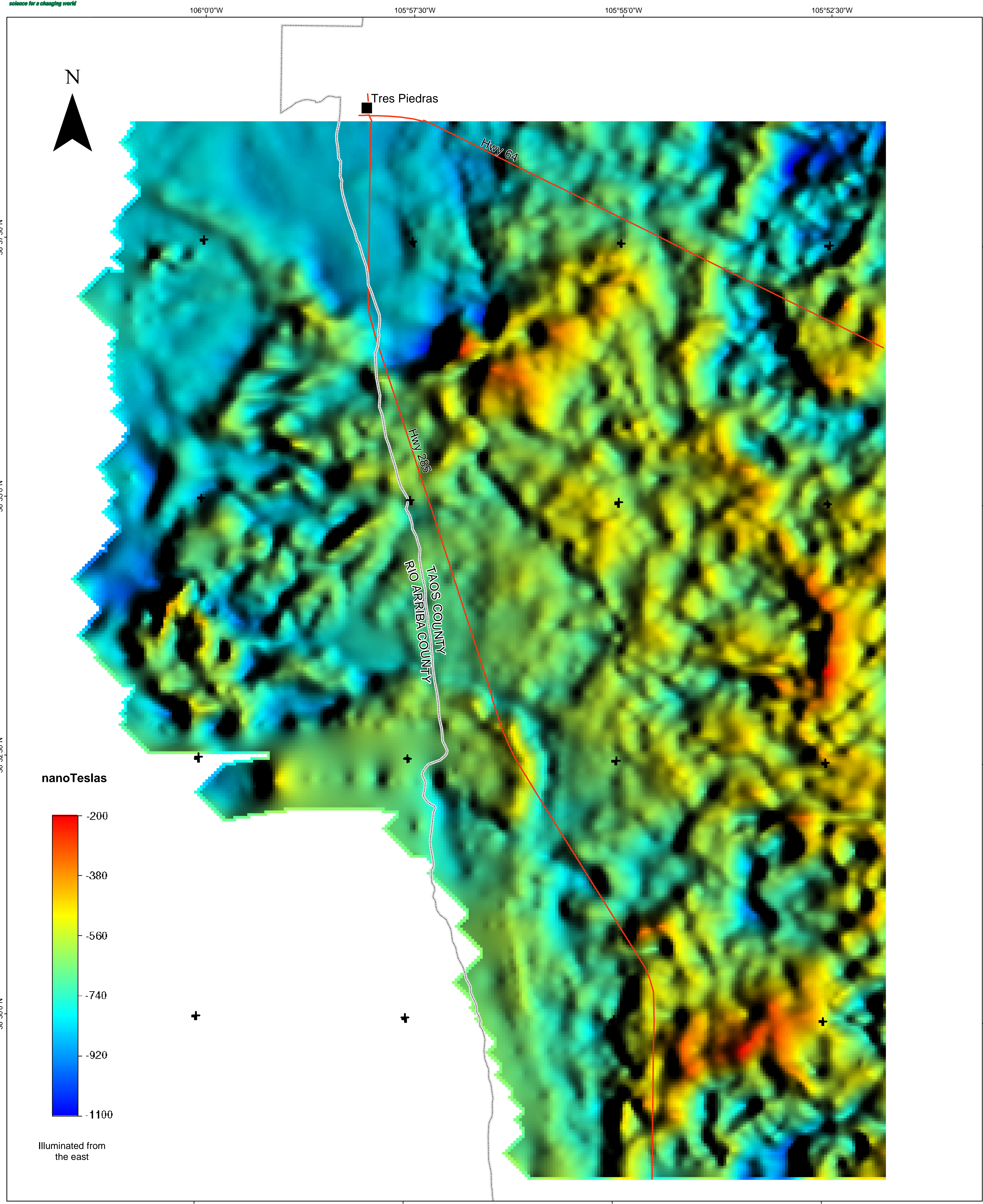
Central San Luis Basin Aeromagnetic Survey Color shaded-relief image of continued, reduced-to-pole (RTP) magnetic data, Petaca Peak area.
