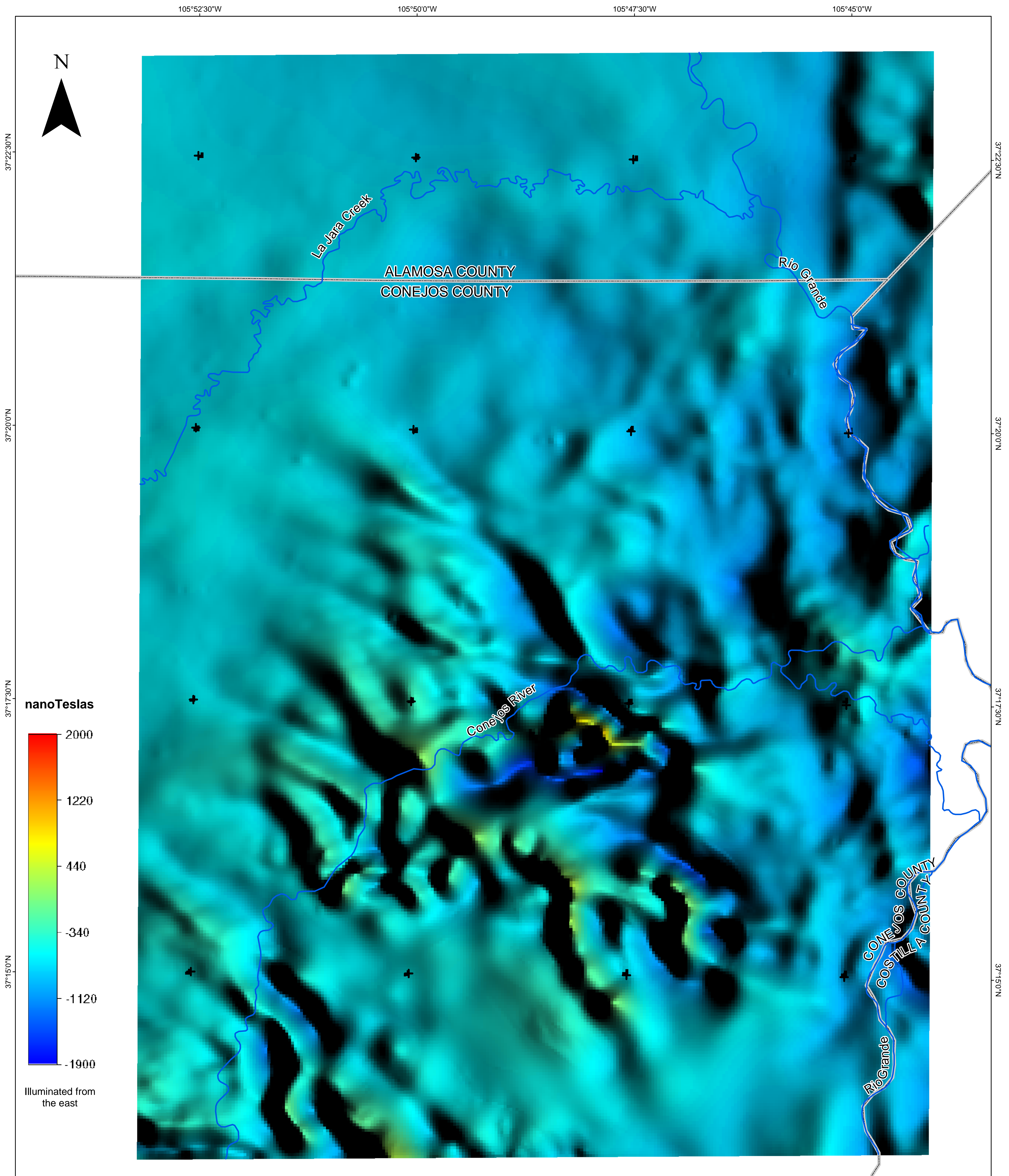
Central San Luis Basin Aeromagnetic Survey Color shaded-relief image of continued, reduced-to-pole (RTP) magnetic data, Pikes Stockade area.
