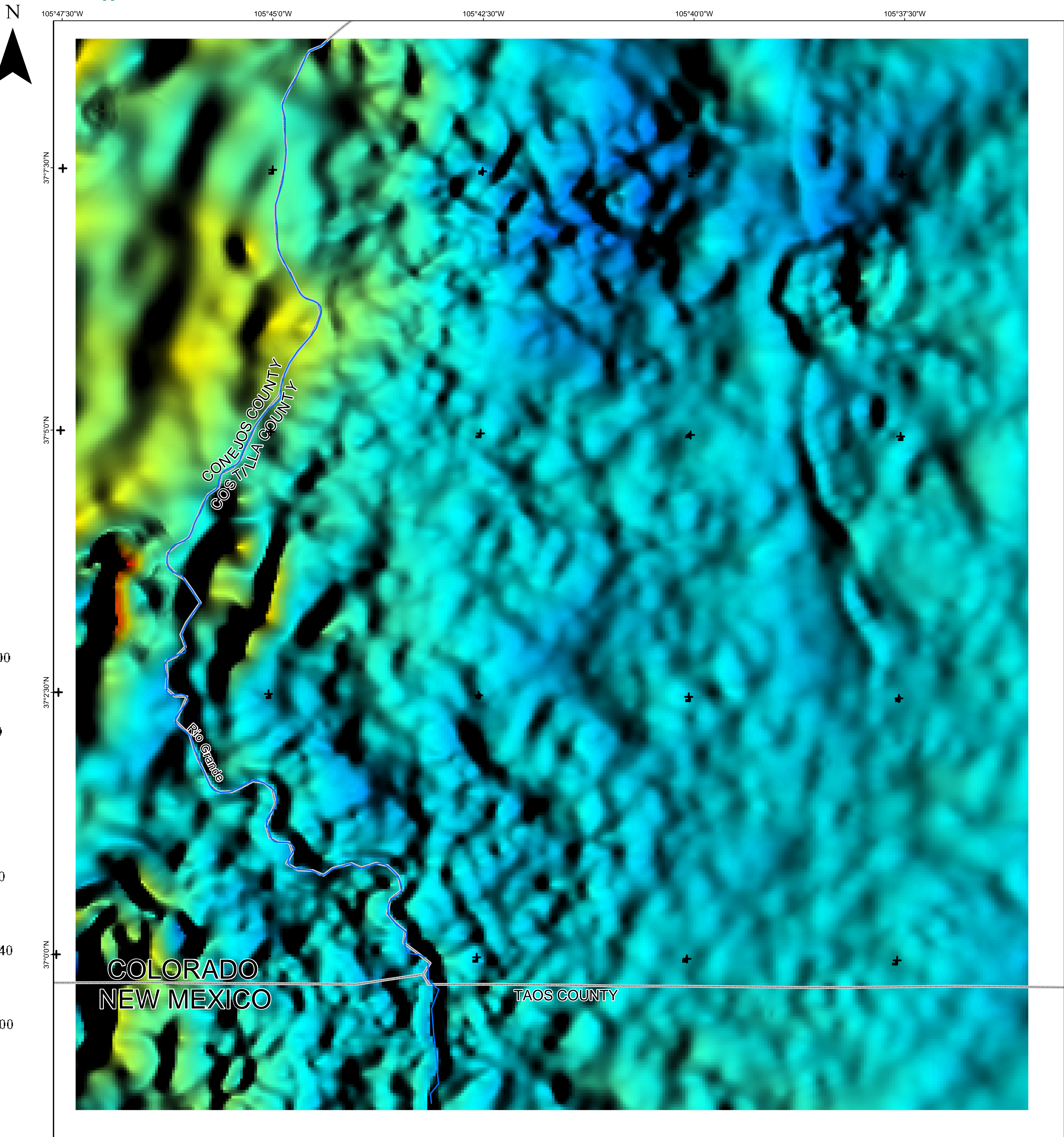
Central San Luis Basin Aeromagnetic Survey Color shaded-relief image of continued, reduced-to-pole (RTP) magnetic data, Sky Valley Ranch area.
