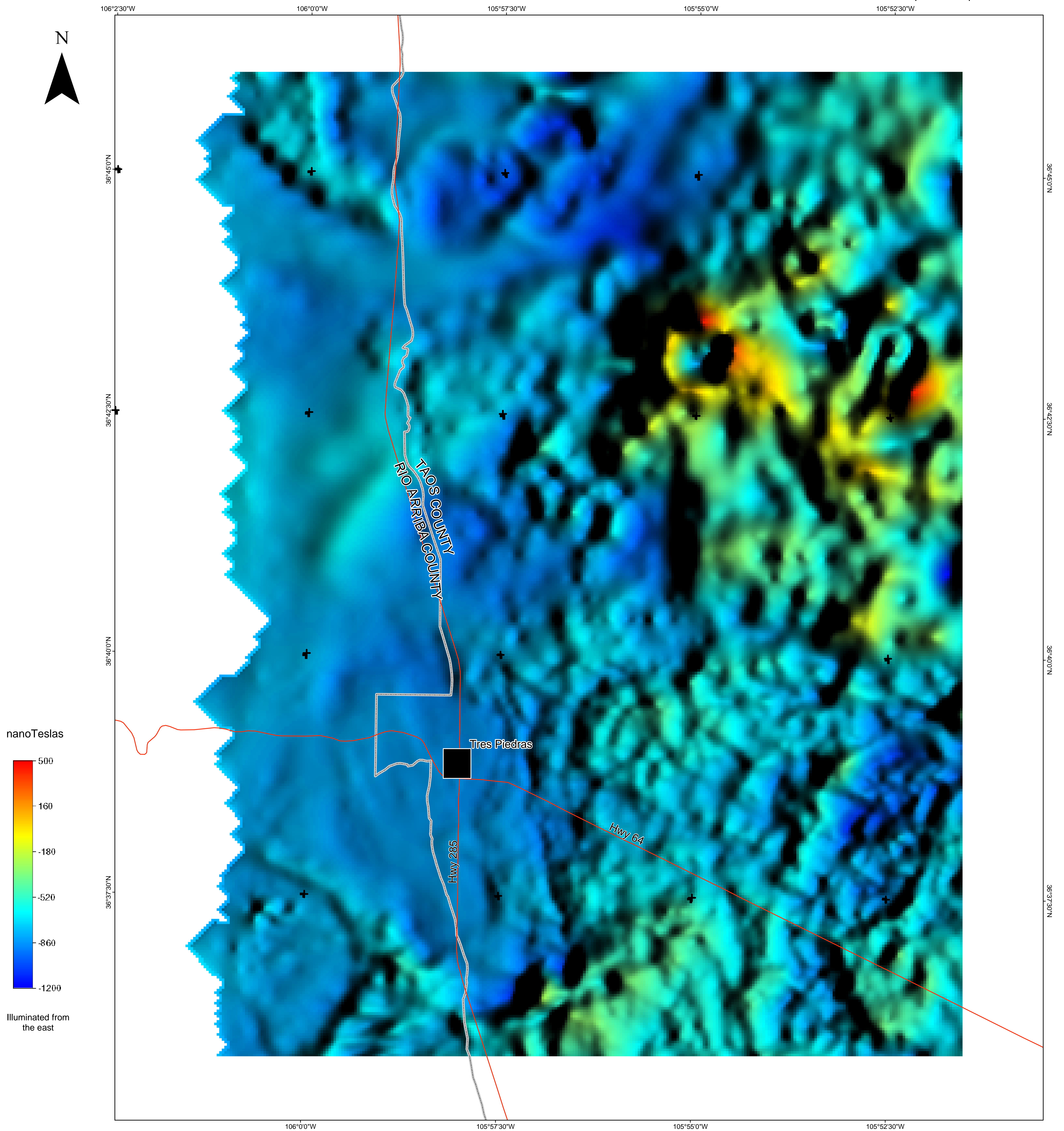
Central San Luis Basin Aeromagnetic Survey Color shaded-relief image of continued, reduced-to-pole (RTP) magnetic data, Tres Piedras area.
