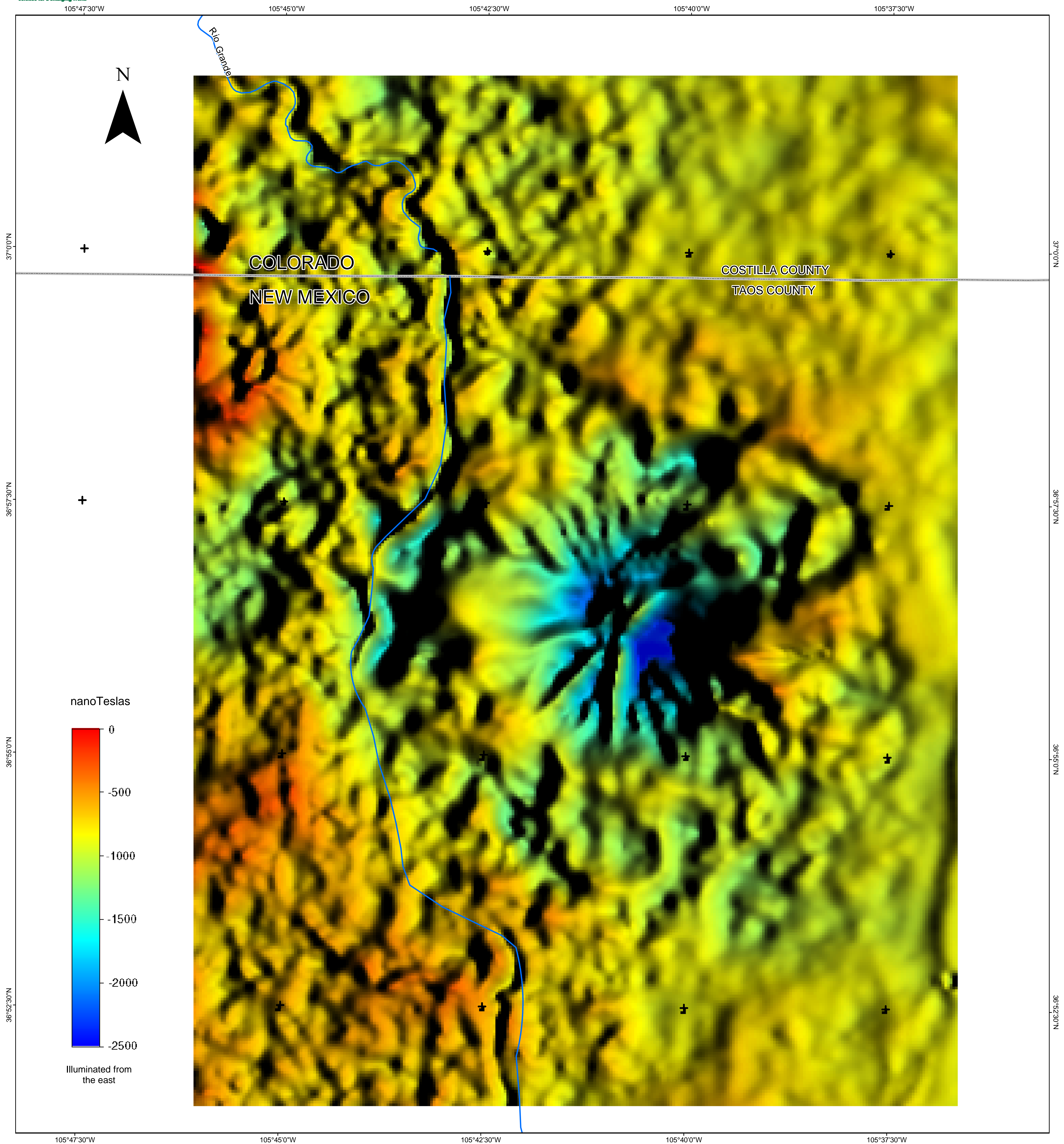
Central San Luis Basin Aeromagnetic Survey Color shaded-relief image of continued, reduced-to-pole (RTP) magnetic data, Ute Mountain area.
