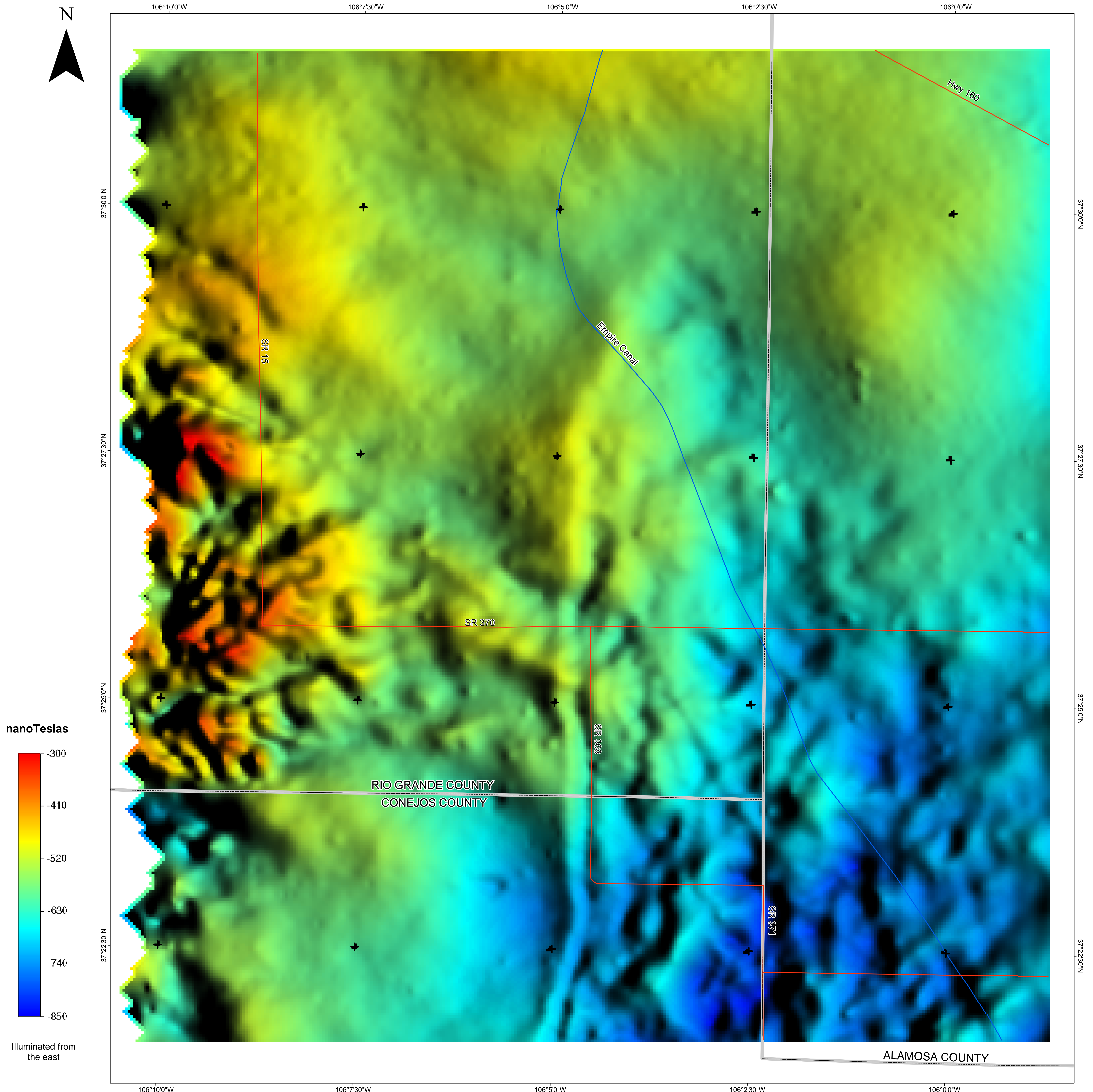
Central San Luis Basin Aeromagnetic Survey Color shaded-relief image of continued, reduced-to-pole (RTP) magnetic data, Waverly area.
