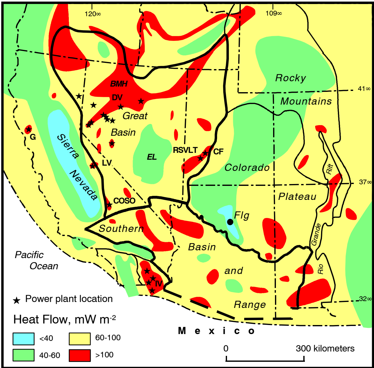
Figure 1. Generalized heat-flow contours for the southwestern United States. BMH, Battle Mountain High; EL, Eureka Low; IV, Imperial Valley.
