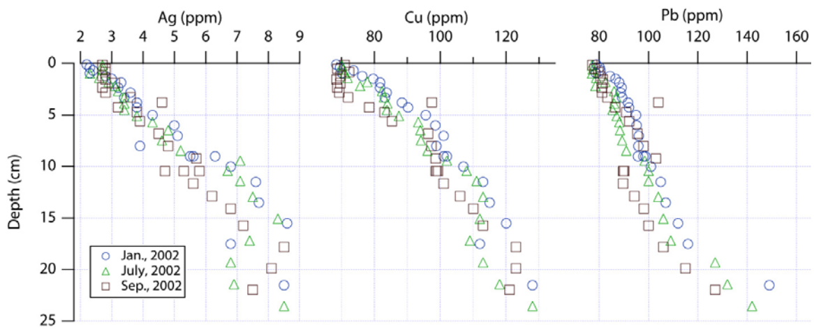
Figure 10.4. Solid phase metal profiles from the Hingham Bay site. Metal concentrations at ~15cm are similar to surface concentrations measured at the same site in 1978 (Bothner and others, 1998). Present concentrations in surface sediments are much lower, but remain high enough to risk negative impacts.
