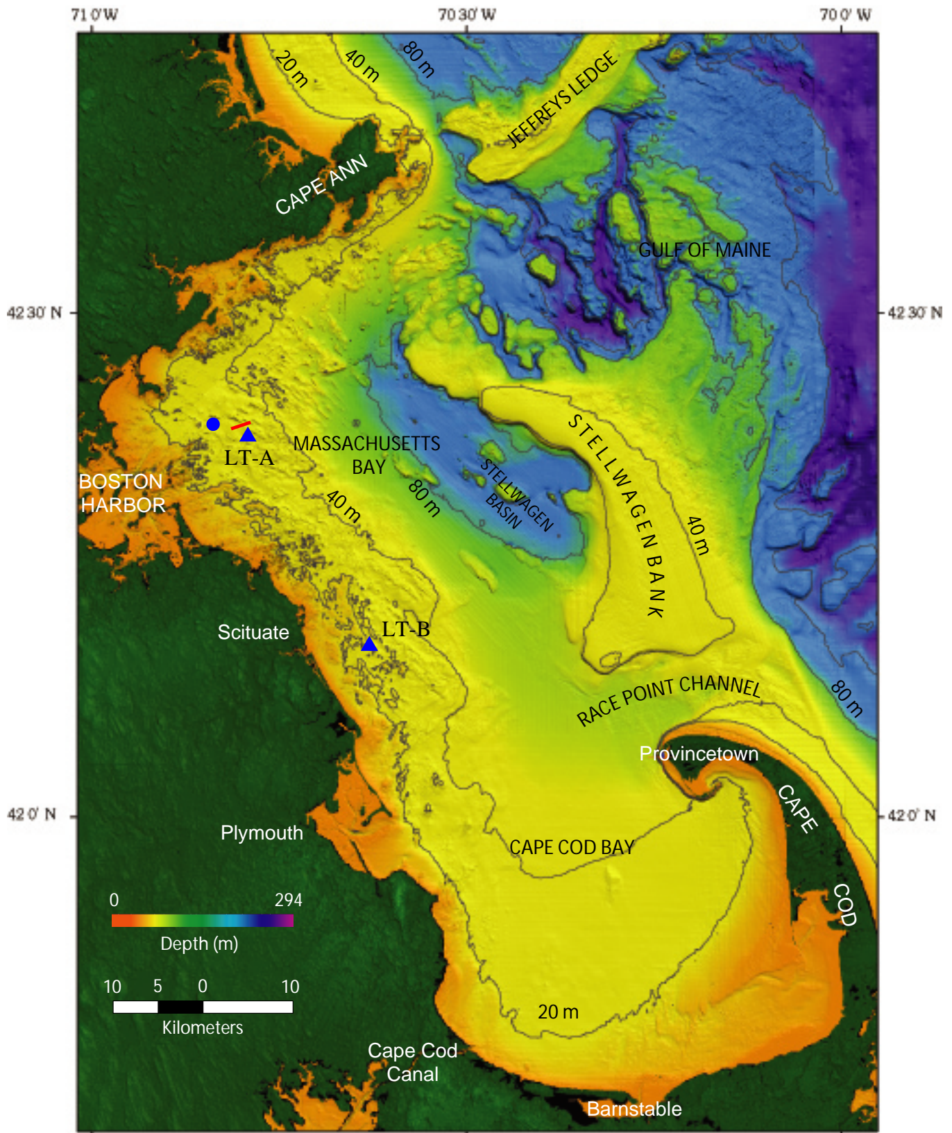
Figure 1.5. Map showing the shaded relief topography, colored by water depth, of the Massachusetts Bay region offshore of Boston, Massachusetts. The location of the diffuser of MWRA ocean outfall is shown as a red line, the USGS long-term oceanographic stations LT-A and LT-B as blue triangles, and the USGS long-term sediment sampling station as a blue circle.
