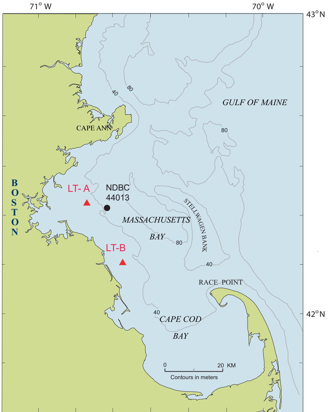
Figure 3.1. The location of long-term oceanographic moorings LT-A and LT-B in western Massachusetts Bay. The LT-A mooring is about 1 km south of the new ocean outfall in about 33 m water depth. The mooring at LT-B is in about 22 m water depth about 5 km offshore. NDBC 44013 is the location of the National Data Buoy Center discus buoy where meteorological observations are obtained. Prior to 1994, these meteorological measurements were made from the USCG Large Navigational Buoy maintained near LT-A.
