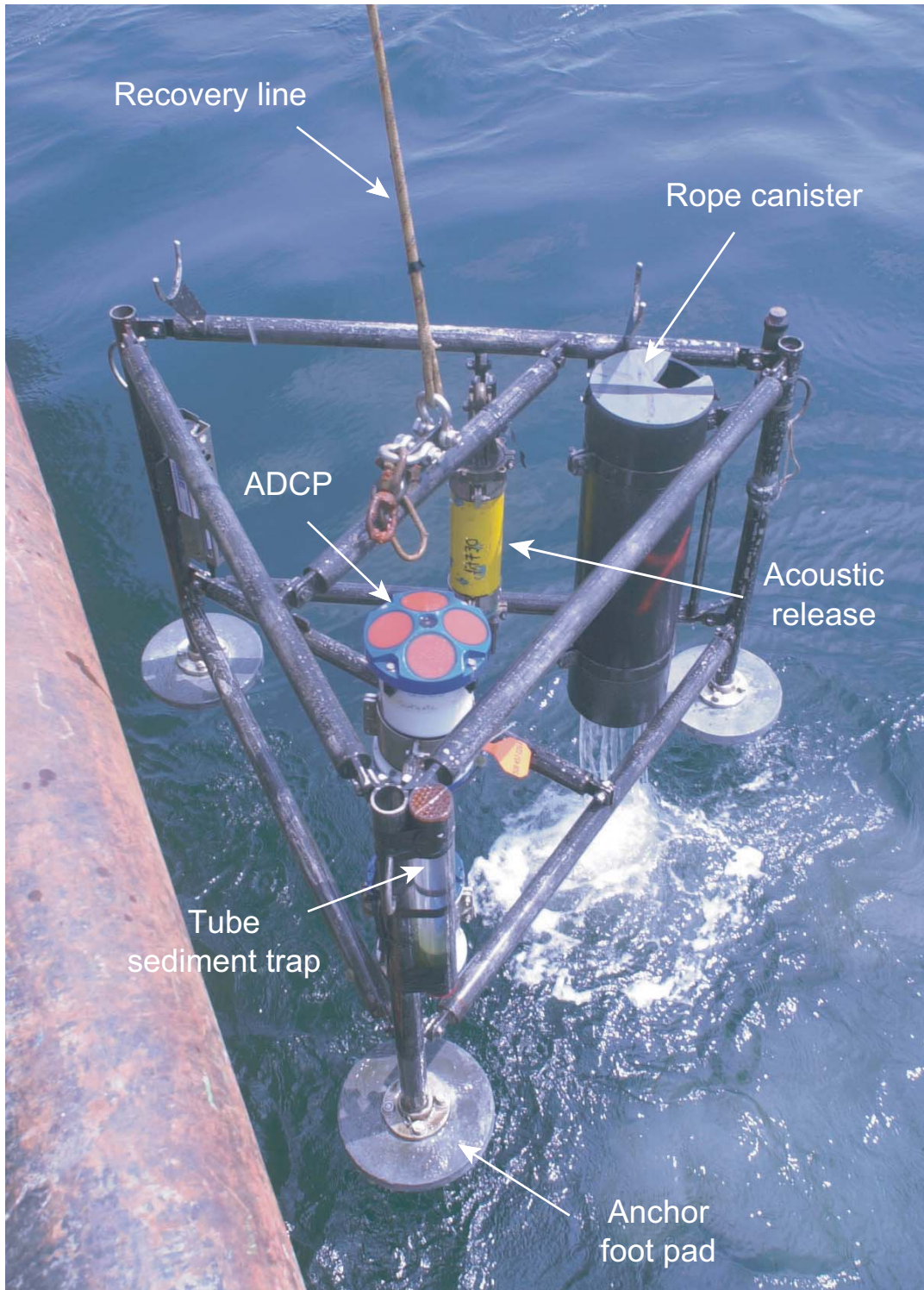
Figure 3.3b. Photograph of an acoustic Doppler current profiler (ADCP) mounted on a small tripod frame being recovered at LT-B. The upward-looking ADCP, mounted in a corner of the frame, has two pairs of transducers that remotely measure currents throughout the water column.
