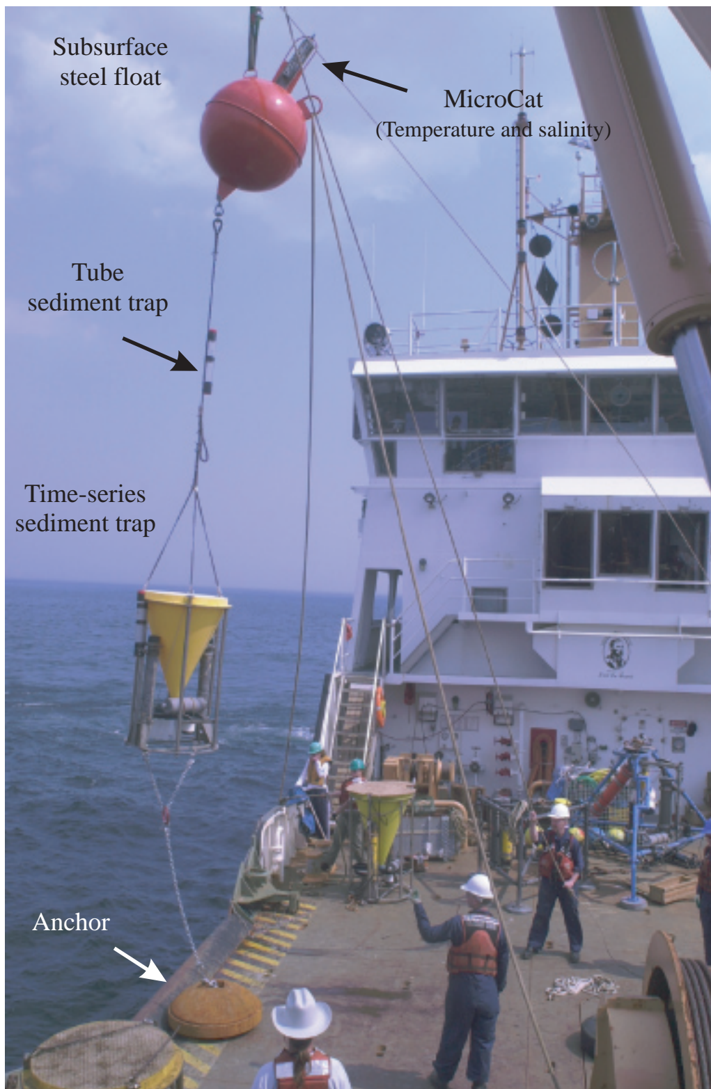
Figure 3.4. A subsurface mooring being deployed from the U.S. Coast Guard Cutter Marcus Hannah at LT-B.
