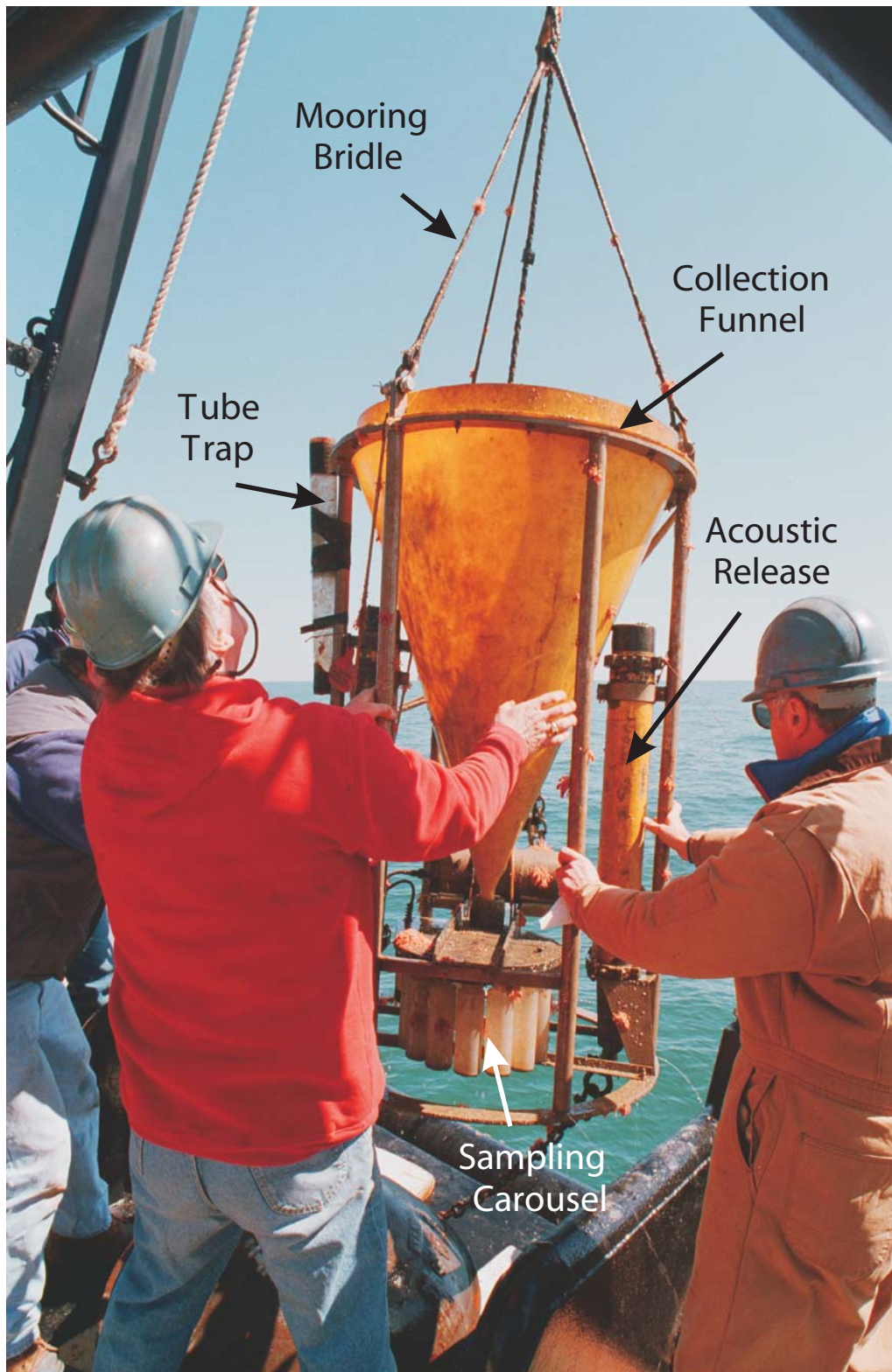
Figure 3.5. Photograph of a Honjo time-series sediment trap. These traps are deployed at Massachusetts Bay long-term sites LT-A and LT-B. The yellow funnel (0.8 m diameter) directs suspended material into one of 13 plastic jars (500 ml capacity), which are sequentially moved under the funnel for a 9-day interval during a typical 4-month deployment.
