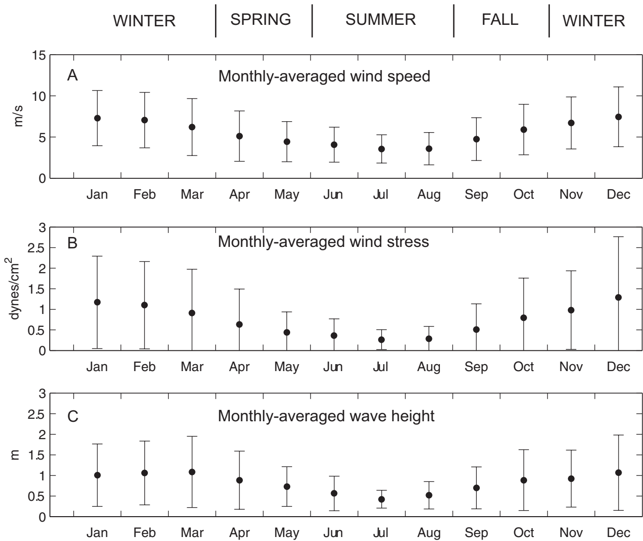
Figure 4.1. Monthly-averaged wind speed (a), magnitude of low-passed wind stress (b), and wave height (c) at NOAA Buoy 44013 (see Figure 3.1 for location). Vertical bars are plus and minus one standard deviation around the mean value (dot).
