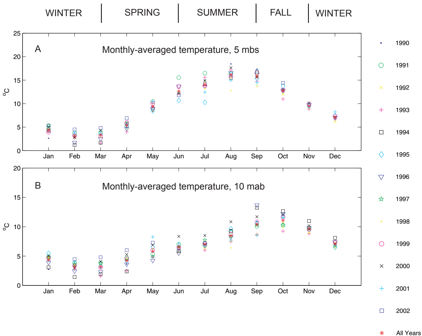
Figure 4.2. Monthly-averaged water temperature at 5 meters below surface (a) and at 10 meters above bottom (b) at the USGS-MWRA long-term monitoring site in western Massachusetts Bay (from Butman and others, 2004a).
