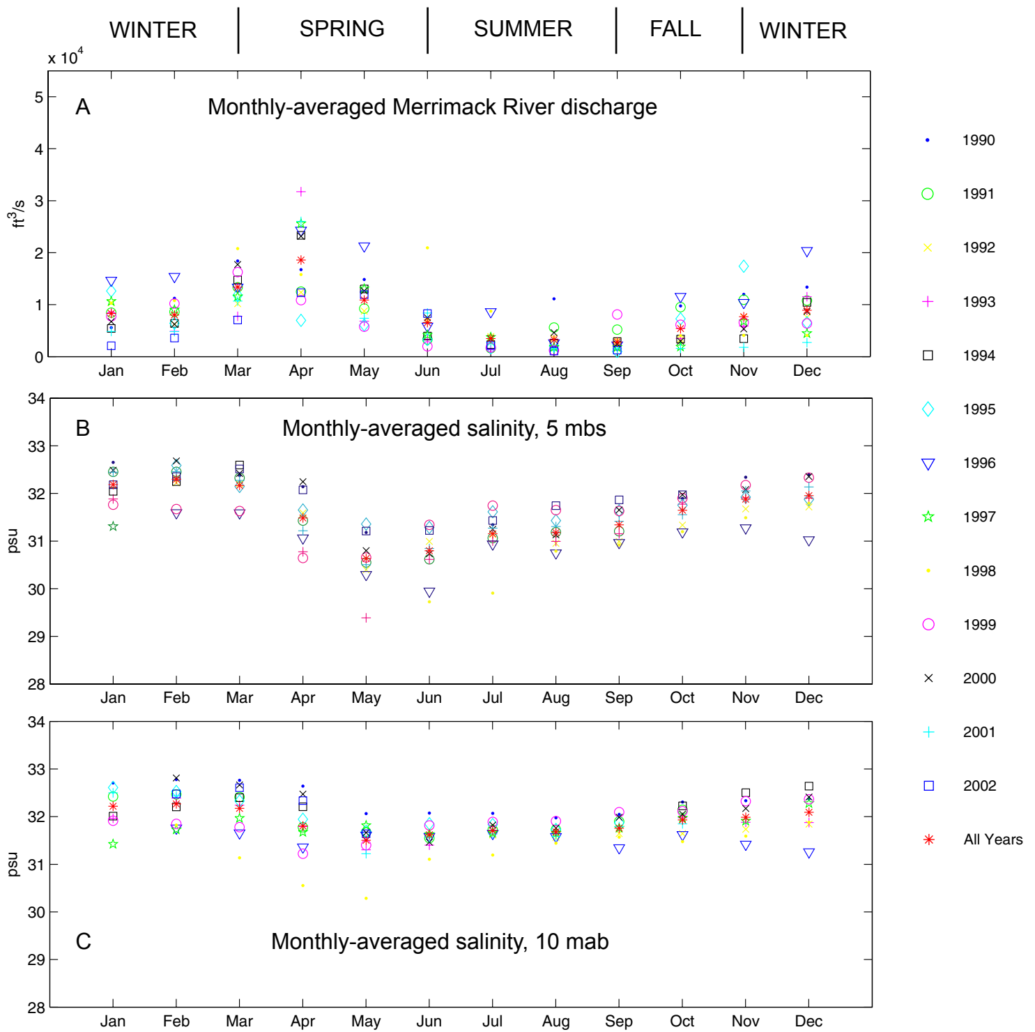
Figure 4.3. Monthly-averaged Merrimack River discharge (a), salinity at 5 meters below surface (b), and salinity at 10 meters above bottom (c) at the USGS-MWRA long-term monitoring site in western Massachusetts Bay (from Butman and others, 2004a).
