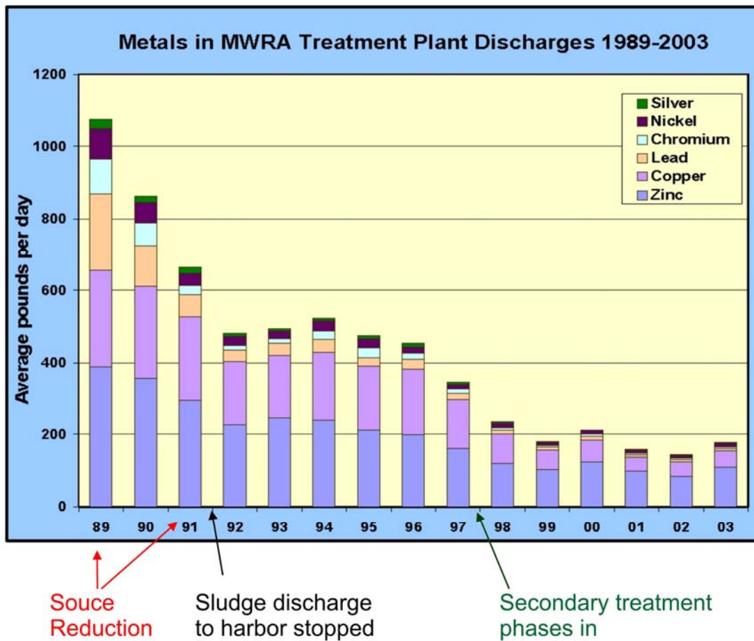
Figure 7.2. Histogram showing the decrease in discharge of metals by the MWRA sewage treatment plants from 1989 to 2003 (Werme and Hunt, 2004).
