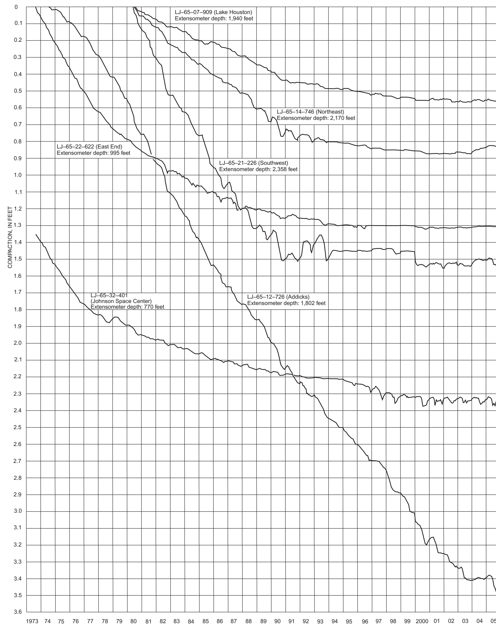
Figure 15. Graphs showing measured compaction of subsurface material, 1973-2005, at borehole extensometer sites shown in figure 14.
