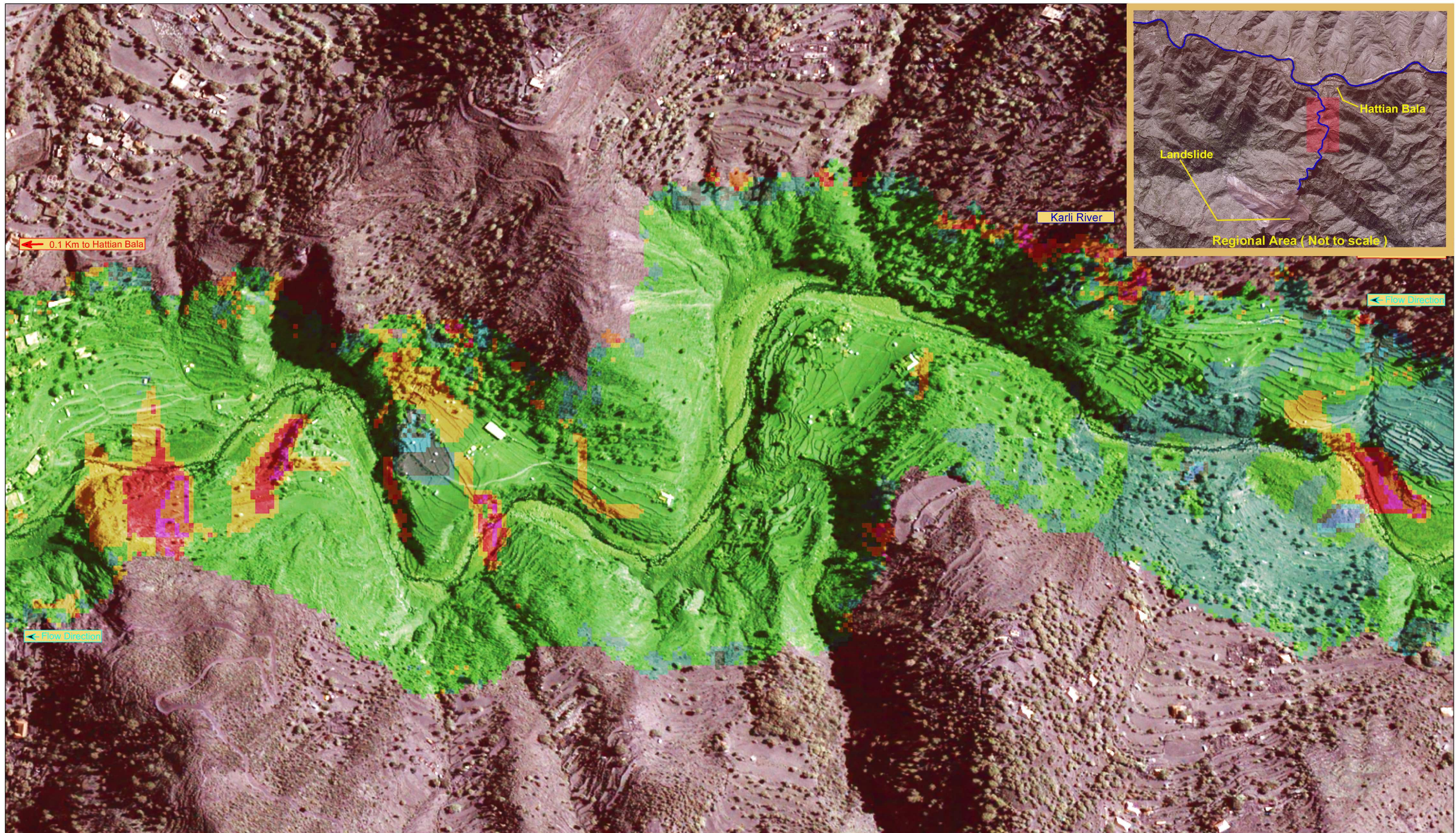
Time to Reach Maximum Inundation Depth Breach Rate: 1000 Meters/Hour (7-meter-deep spillway cut scenario)
