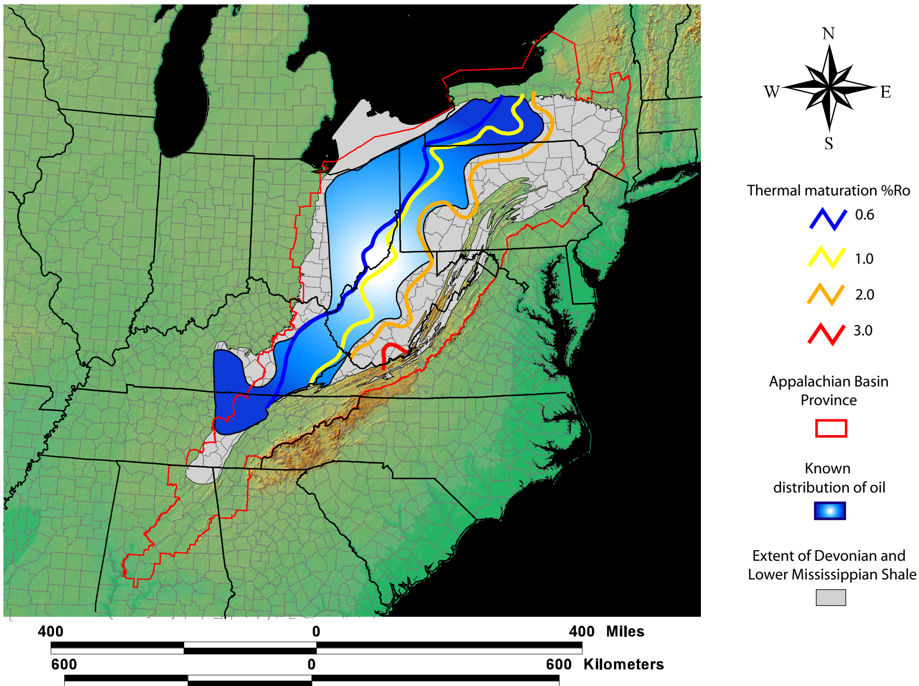
Figure 10. The Appalachian Basin Province, illustrating the extent of the Devonian and Lower Mississippian shale, the limit of generation and preservation of oil in the Devonian shale and Oriskany Sandstone, and vitrinite reflectance (%Ro) isotherm contours (Repetski and others, 2002, 2005; personal communication; Weary and others, 2000, 2001).
