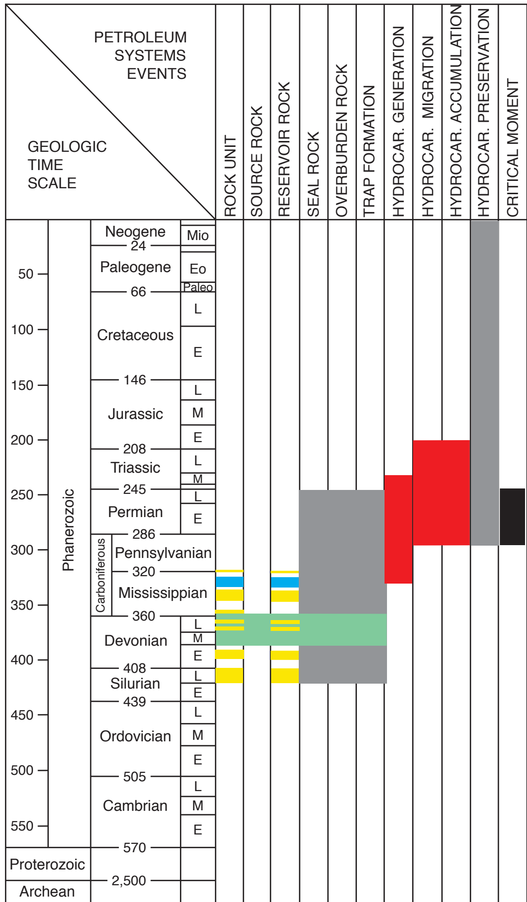
Figure 12. Petroleum system events chart for the Devonian Shale-Middle and Upper Paleozoic Total Petroleum System in the Apalachian basin.
