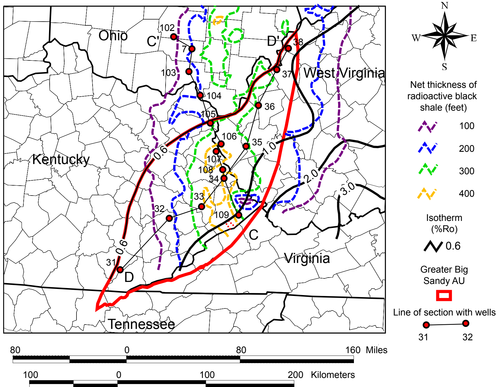
Figure 14. Greater Big Sandy Assessment Unit, showing thermal maturity in %Ro and net thickness of radioactive black shale. Well numbers and lines of cross sections are from de Witt and others (1993). Cross sections CC' and DD' are shown on figures 16 and 17, respectively. See figure 11 for source of %Ro isotherm data.
