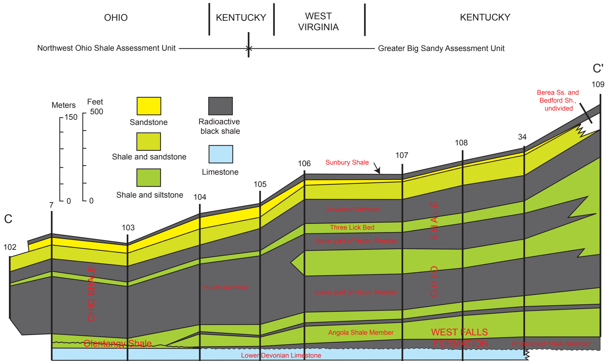
Figure 16. Stratigraphic cross section CC', showing the Devonian black shales across the Greater Big Sandy Assessment Unit in southern Ohio, eastern Kentucky, West Virginia, and southwestern Virginia. Location of cross section is shown on figure 14 (after de Witt and others, 1993, pl. 9, section HH').
