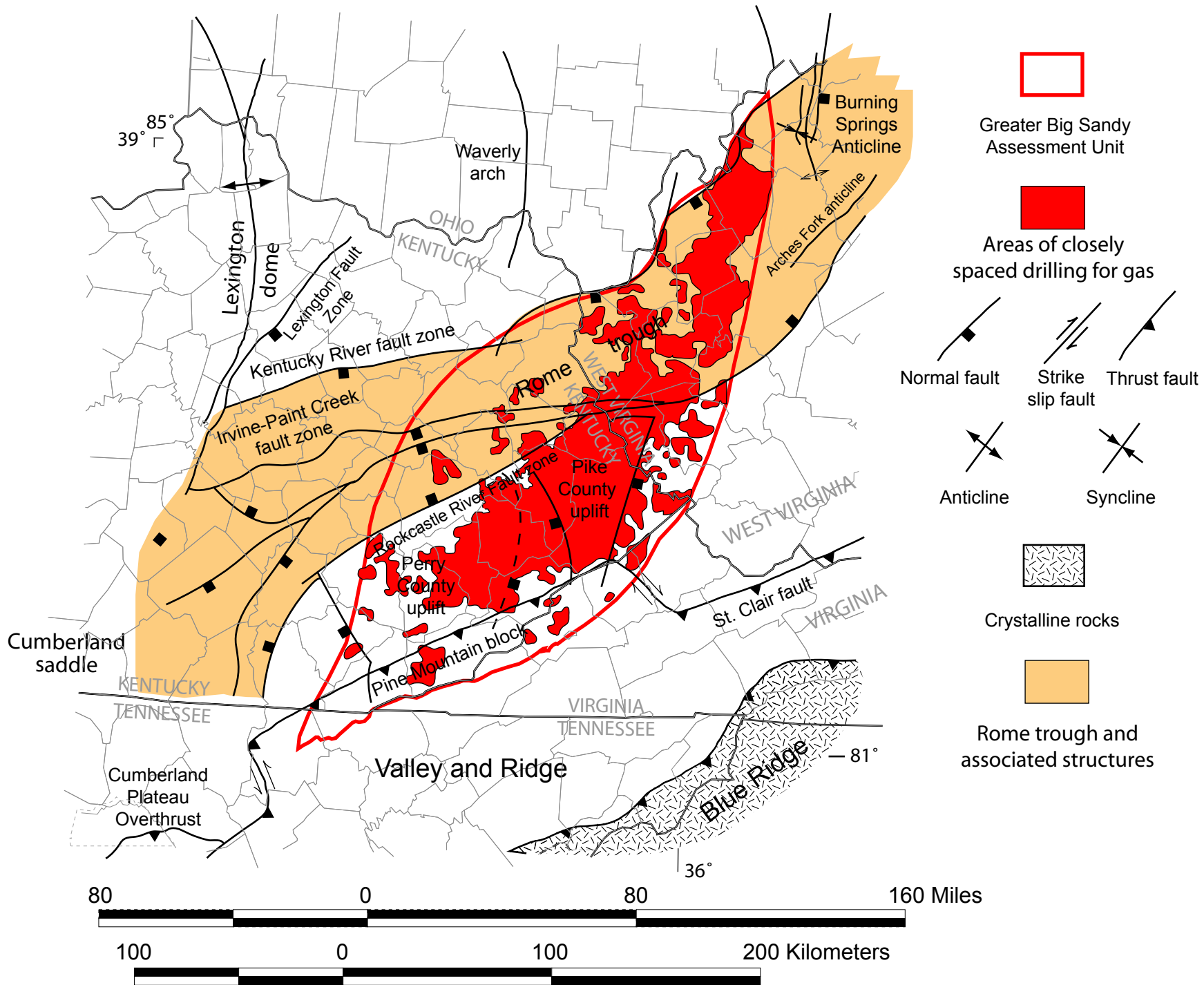
Figure 18. Greater Big Sandy Assessment Unit, showing the relationship of the AU to regional geologic structure (structure adapted from Ryder and others, in press).
