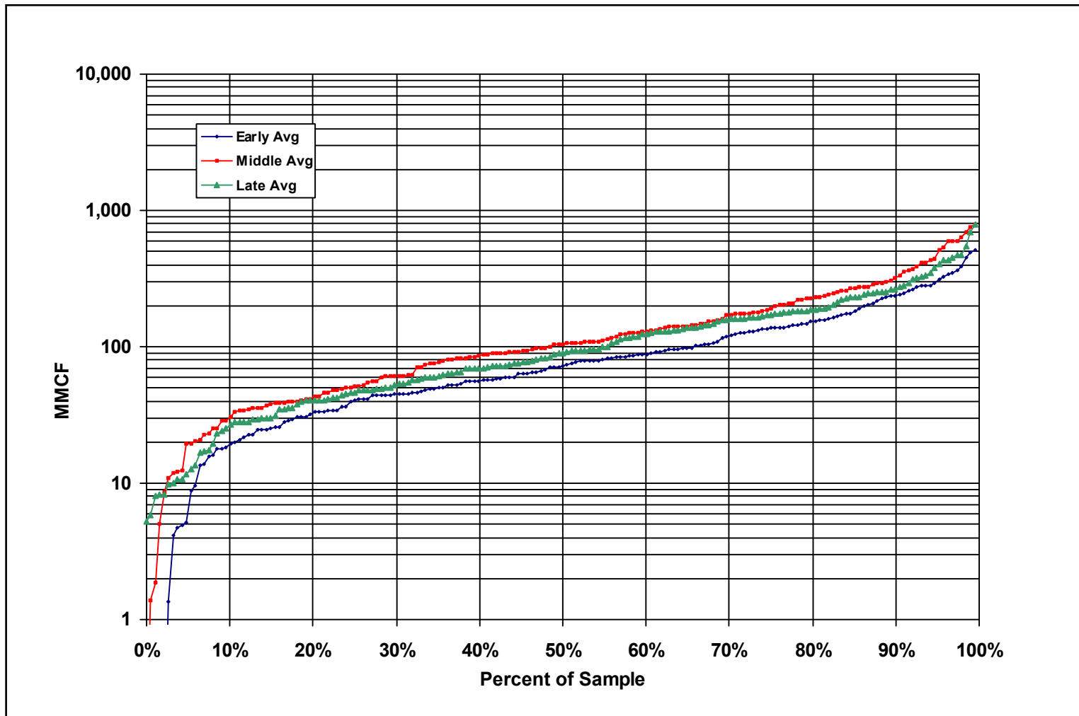
Figure 21. Distribution of Estimated Ultimate Recovery (EUR) values per well for wells in the Devonian shale of eastern Kentucky (by thirds); MMCF is million cubic feet, (Troy Cook, USGS, unpublished data 2002).
