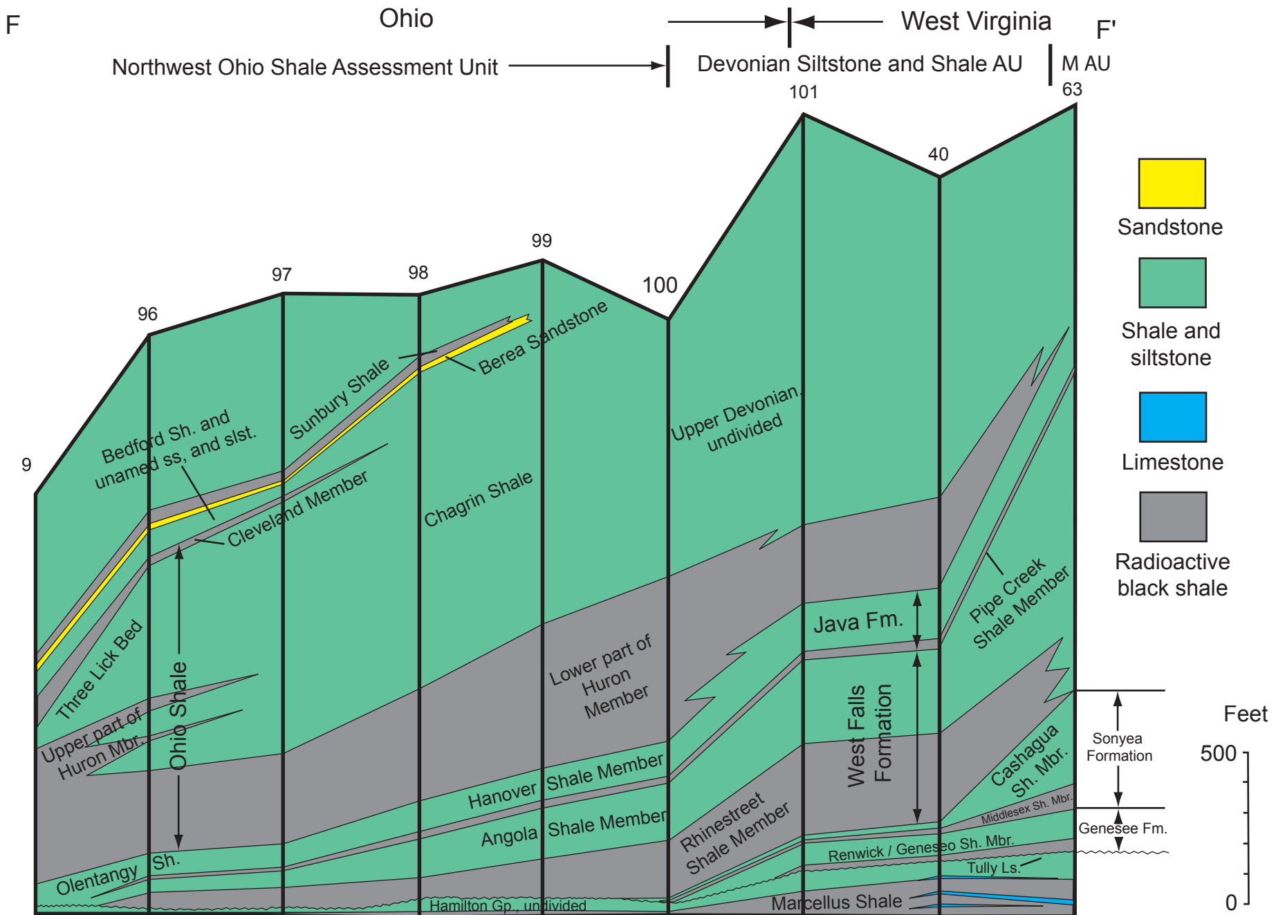
Figure 24. Cross section FF', showing the Devonian black shales across western West Virginia and Ohio (after de Witt and others, 1993, pl. 8, section GG'). Numbers along top of section refer to the well numbers of de Witt and others (1993). M AU is Marcellus Shale Assessment Unit; (see fig. 22 for location).
