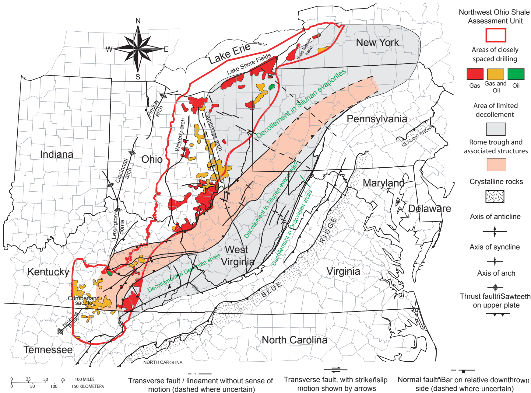
Figure 25. Northwestern Ohio Shale AU showing relationship of hydrocarbon accumulations to geologic structure. Structural geology is adapted from Ryder and others (in press); decollement data are from Colton (1970) and Sanford (1993).
