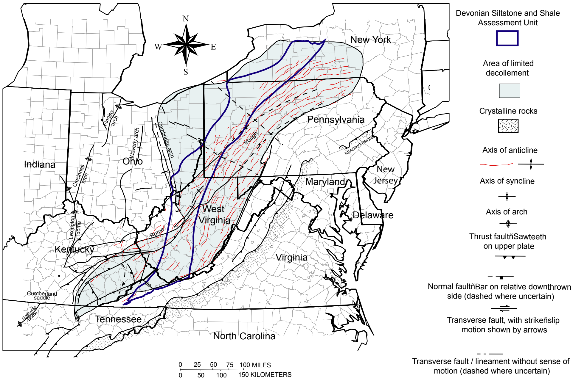
Figure 26. Devonian Siltstone and Shale AU, showing relationship of AU to geologic structure. Structural geology is adapted from Ryder and others (in press); decollement data are from Colton (1970) and Frey (1973).
