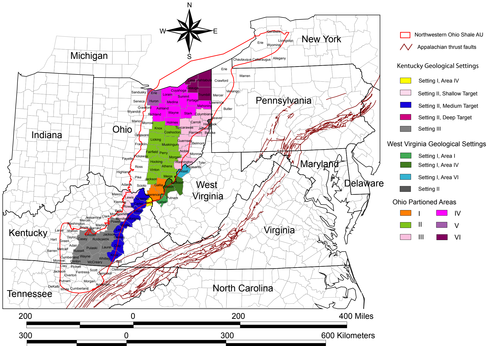
Figure 28. Geological settings and partioned areas in Northwestern Ohio Shale Assessment Unit. Data are from Kuuskraa and Wicks (1984); Kuuskraa and others (1985); and Lewin and Associates (1983); (see Table 8 for resource data).
