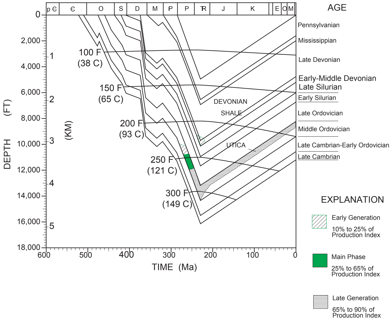
Figure 29. Burial and hydrocarbon generation plot for the Amerada No. 1 Ullman well in Noble County, Ohio; modified slightly from Ryder and others (1998); (see fig. 22 for location of well).
