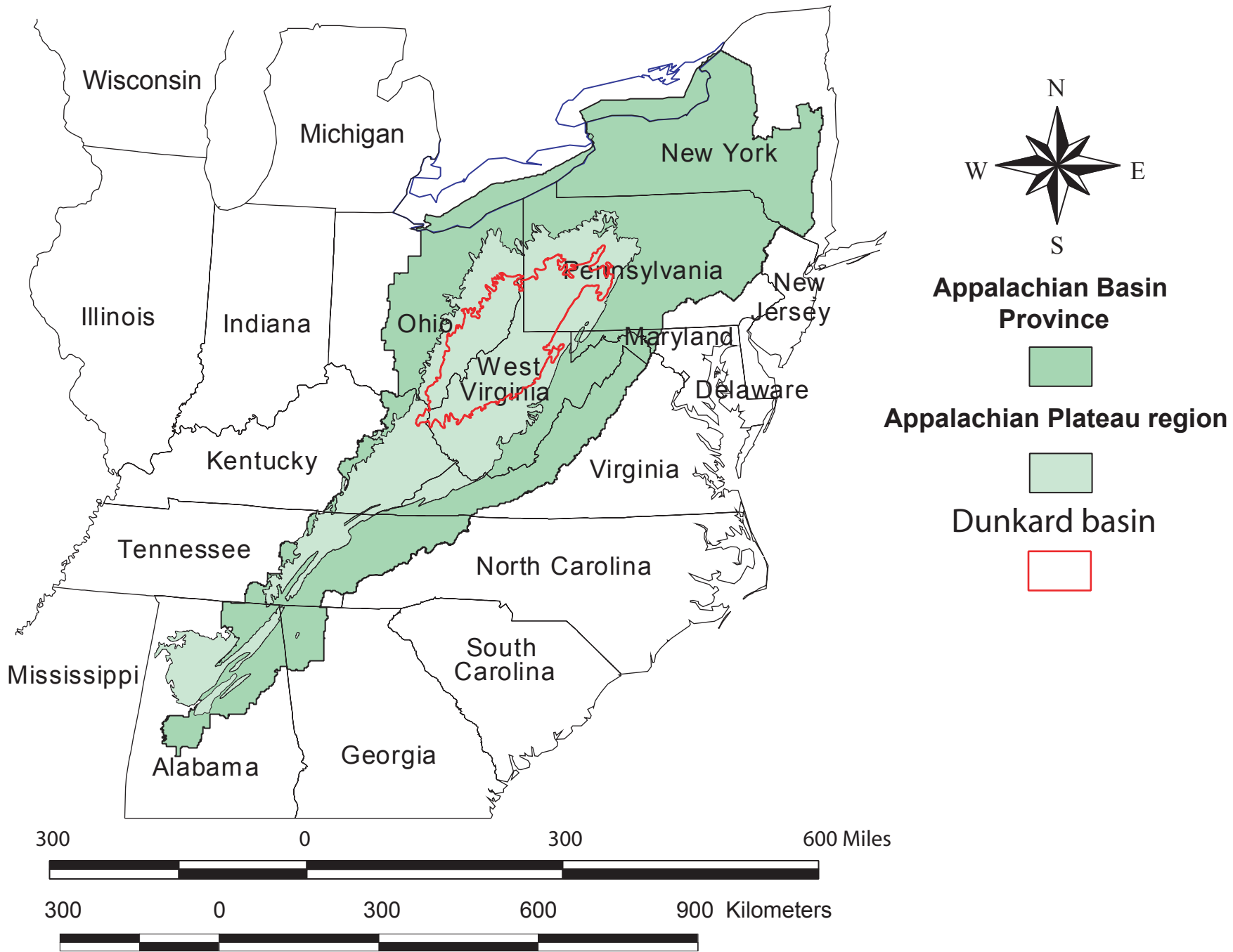
Figure 3. Location of the Appalachian Basin Assessment Province in the United States. The map shows the area of the Appalachian Basin Province assessed by the USGS for hydrocarbons in 1995 (Gautier and others, 1995) and 2002 (Milici and others, 2003).
