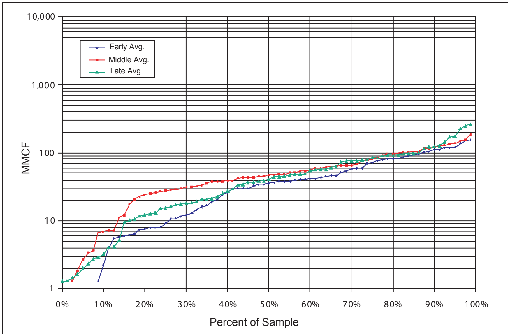
Figure 30. Distribution of Estimated Ultimate Recovery (EUR) values per well, for wells in the northwestern Ohio Shale Assessment Unit (by thirds); MMCF is million cubic feet, (Troy Cook, USGS, unpublished data 2002)
