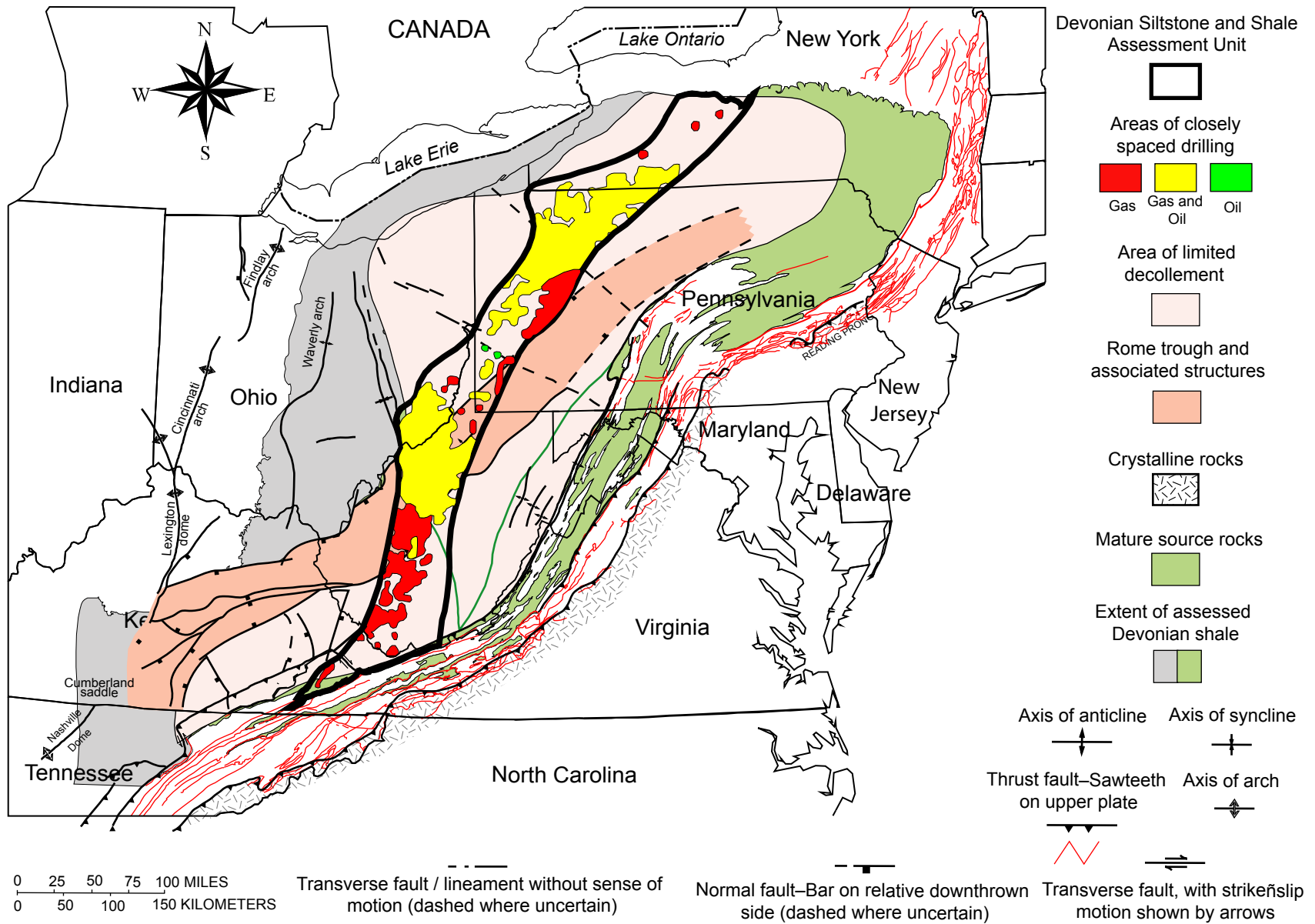
Figure 31. Devonian Siltstone and Shale AU, showing relationship of hydrocarbon accumulations to geologic structure. Structural geology adapted from Ryder and others (in review); decollement data from Colton (1970), and Frey (1973).
