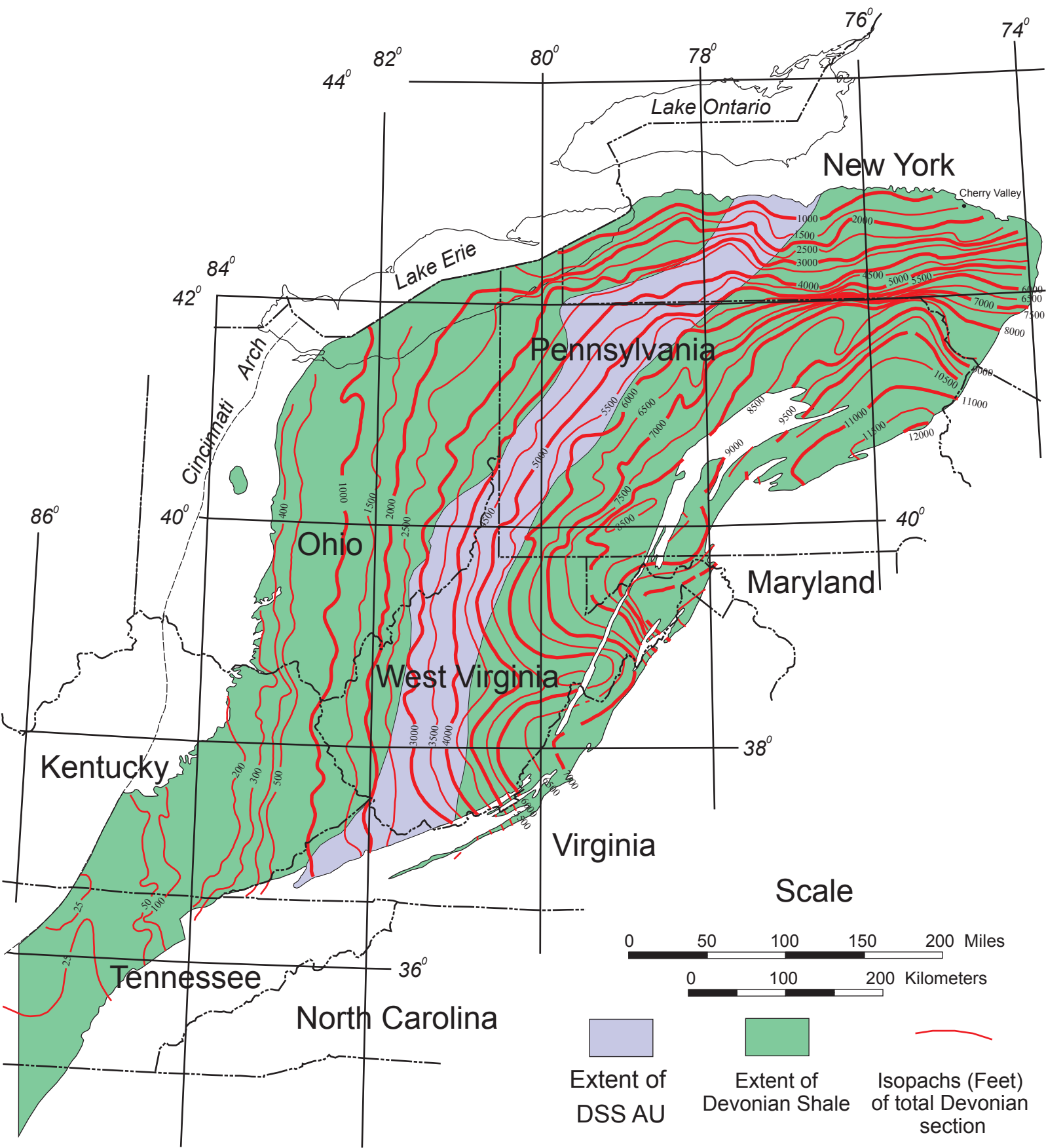
Figure 32. Extent and thickness of Devonian rocks in the Appalachian basin, showing the location of the Devonian Siltstone and Shale AU (adapted from de Witt and others, 1975).
