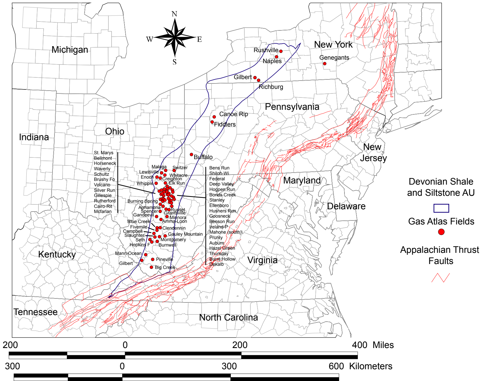
Figure 33. Named fields in the Devonian Siltstone and Shale and Marcellus Shale Assessment Units; (data from Roen and Walker, 1996).
