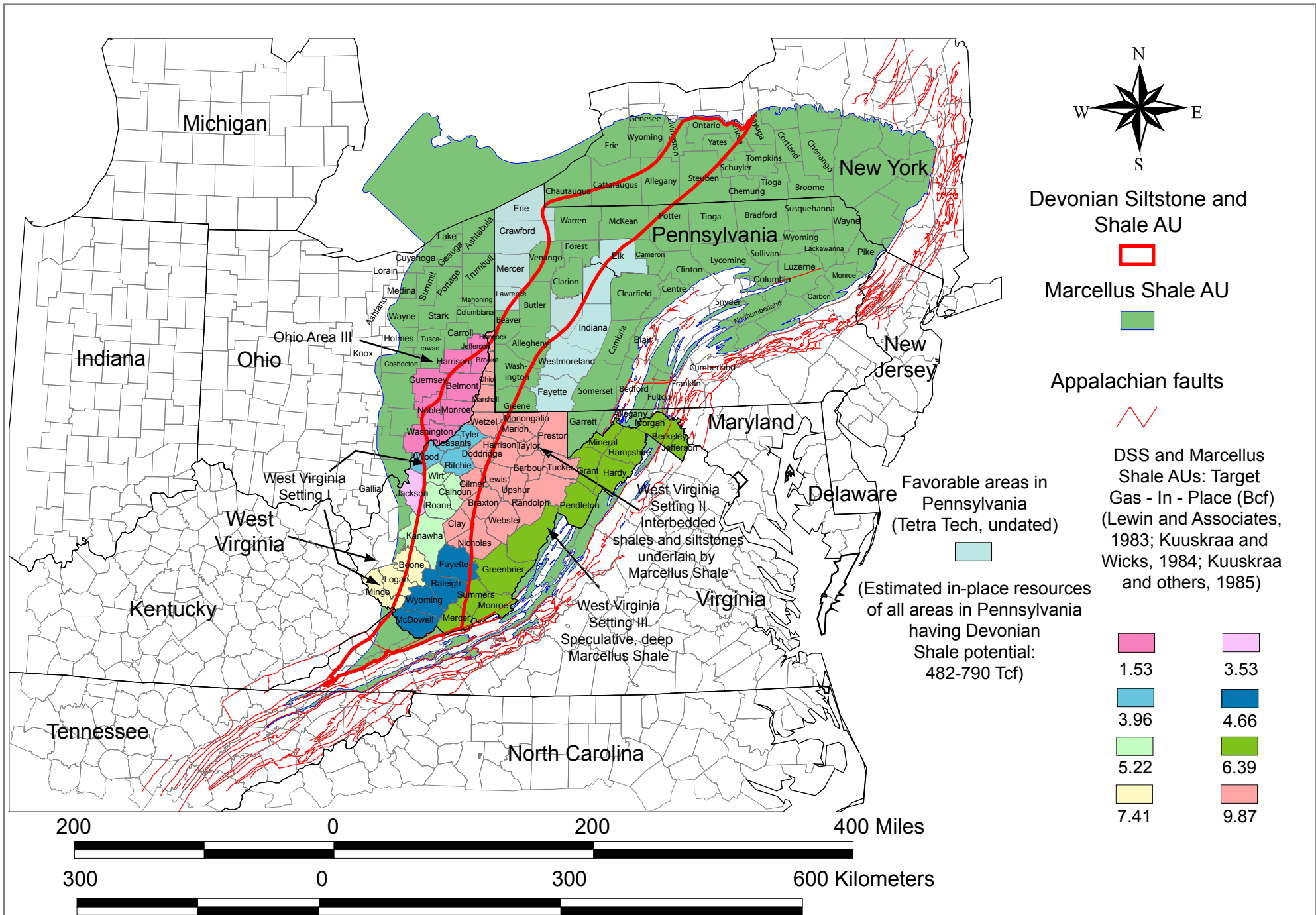
Figure 34. In-place gas resource estimates for target shale formations (Huron, Rhinestreet, Marcellus) in areas of Devonian Siltstone and Shale and Marcellus Shale Assessment Units. Data are from Lewin and Associates (1983); Kuuskraa and Wicks (1984); Kuuskraa and others (1985); and Tetra Tech (undated).
