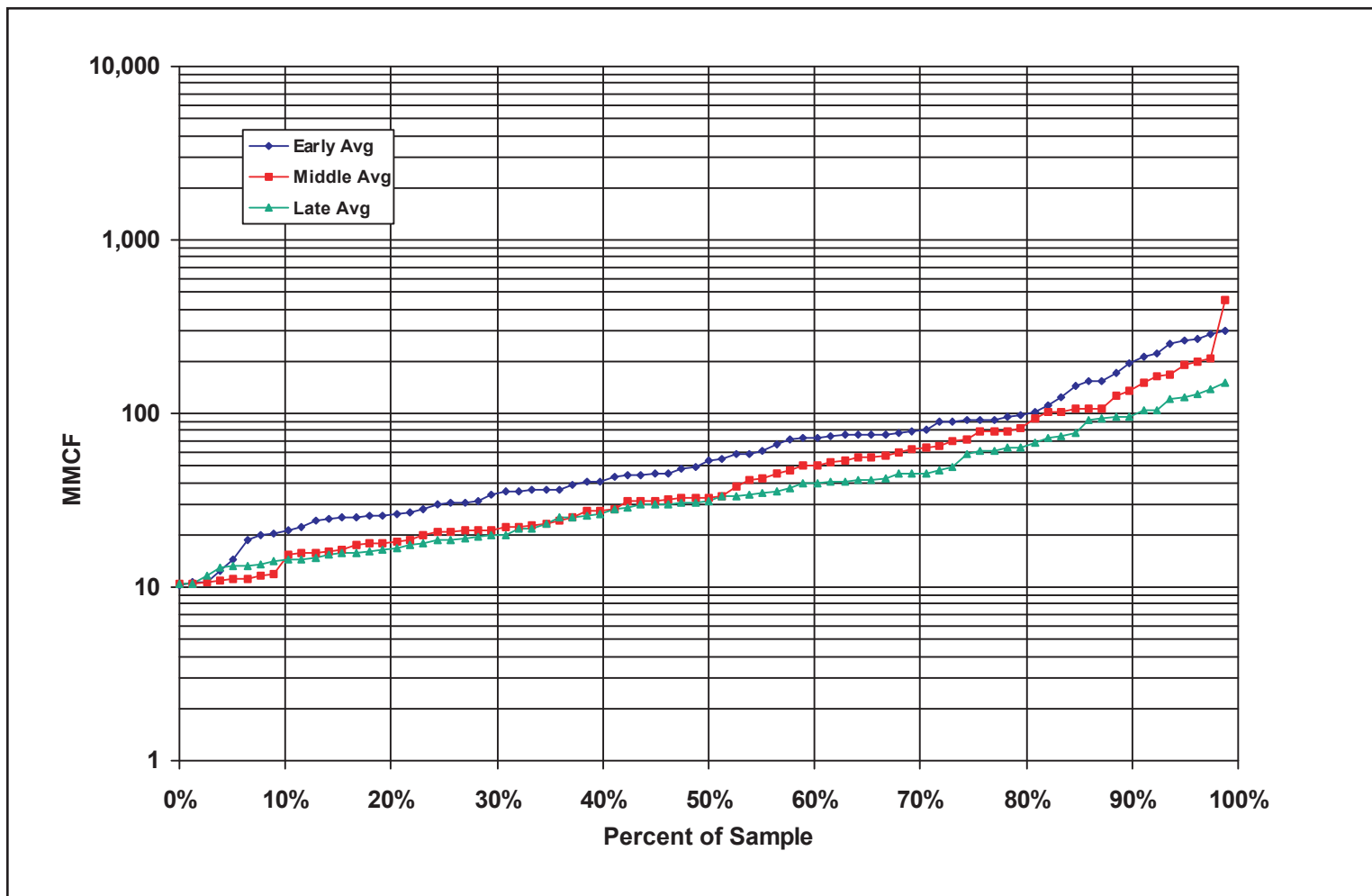
Figure 35. Distribution of Estimated Ultimate Recovery (EUR) values per well for wells for the Devonian Siltstone and Shale Assessment Unit (by thirds); MMCF is million cubic feet (Troy Cook, USGS, unpublished data 2002).
