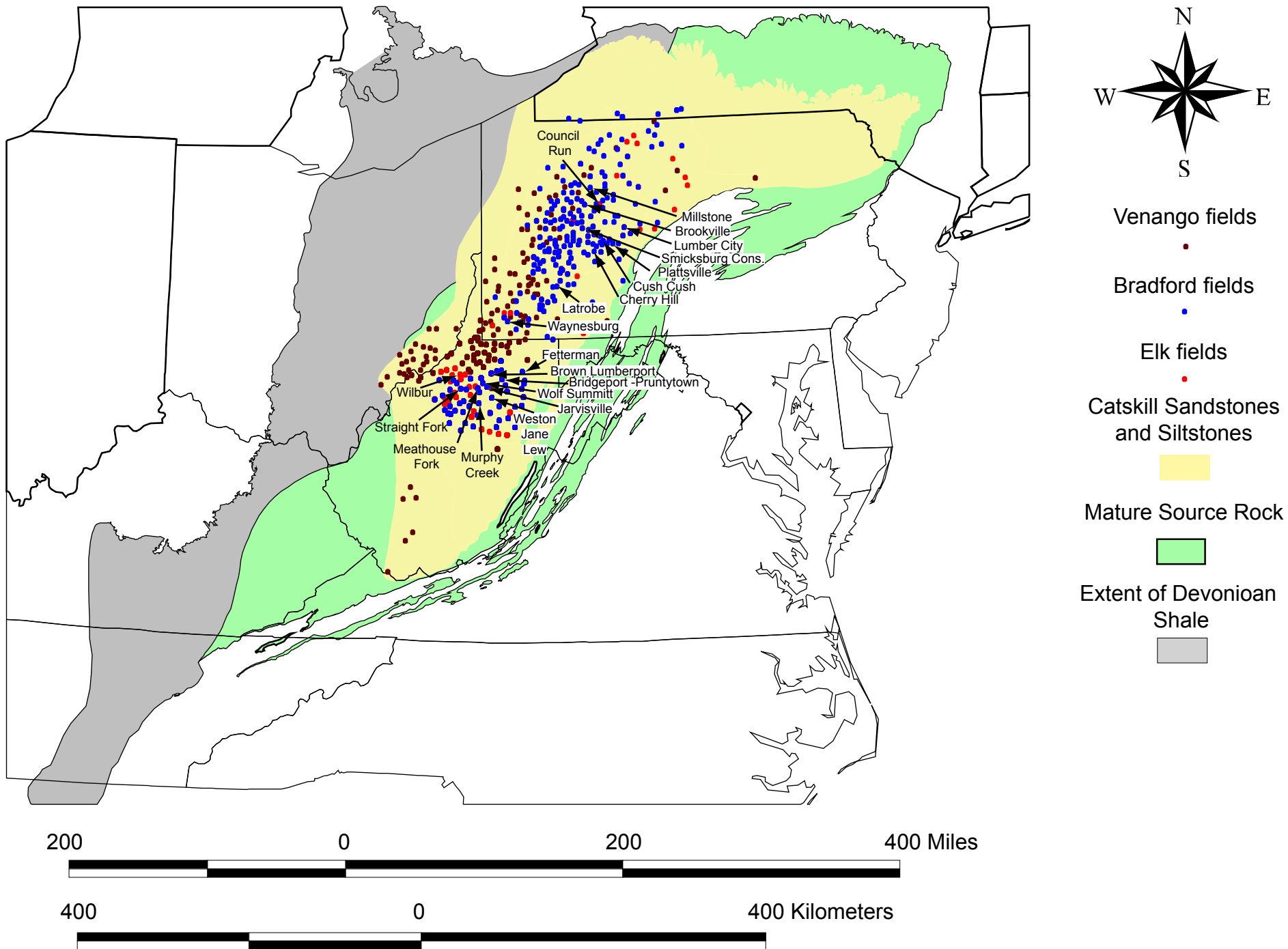
Figure 37. Catskill Sandstones and Siltstones Assessment Unit, showing distribution of Elk, Bradford, and Venango fields and selected field names (from Boswell, Heim, and others, 1996; Boswell, Thomas, and others, 1996; Donaldson and others, 1996).
