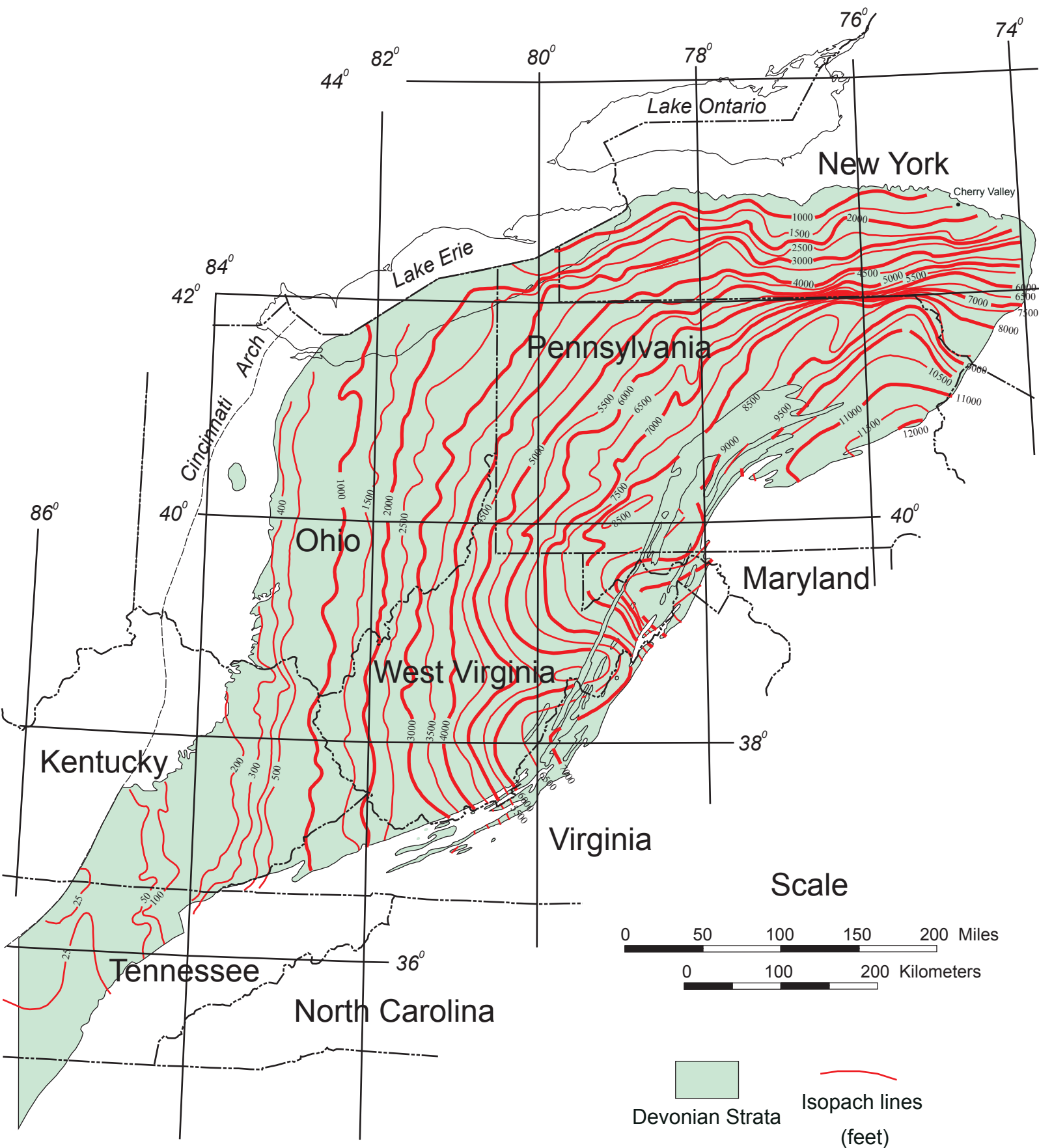
Figure 4. Extent and thickness of Devonian rocks in the U.S. part of the Appalachian basin east of the Cincinnati arch (adapted from deWitt and others, 1975).
