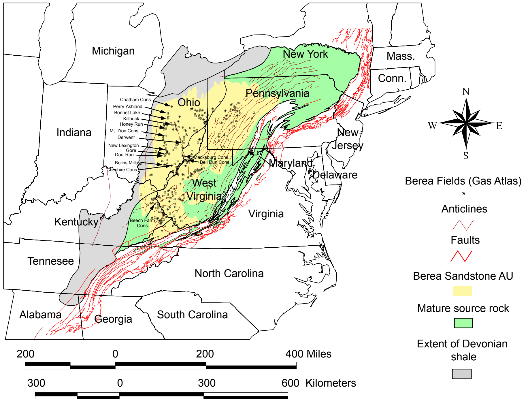
Figure 43. The Berea Sandstone AU, showing gas-producing fields (data from Roen and Walker, 1996).
