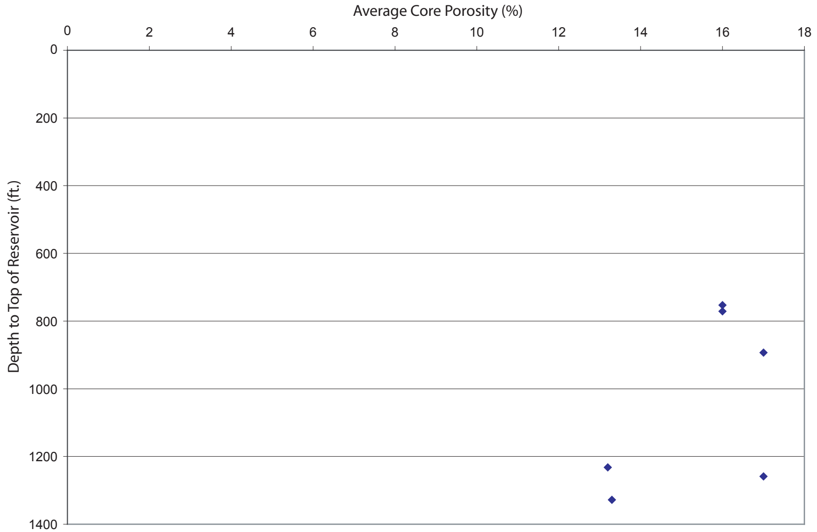
Figure 44. Graph of Berea Sandstone average core porosity vs. depth to top of reservoir (data from Table 11).
