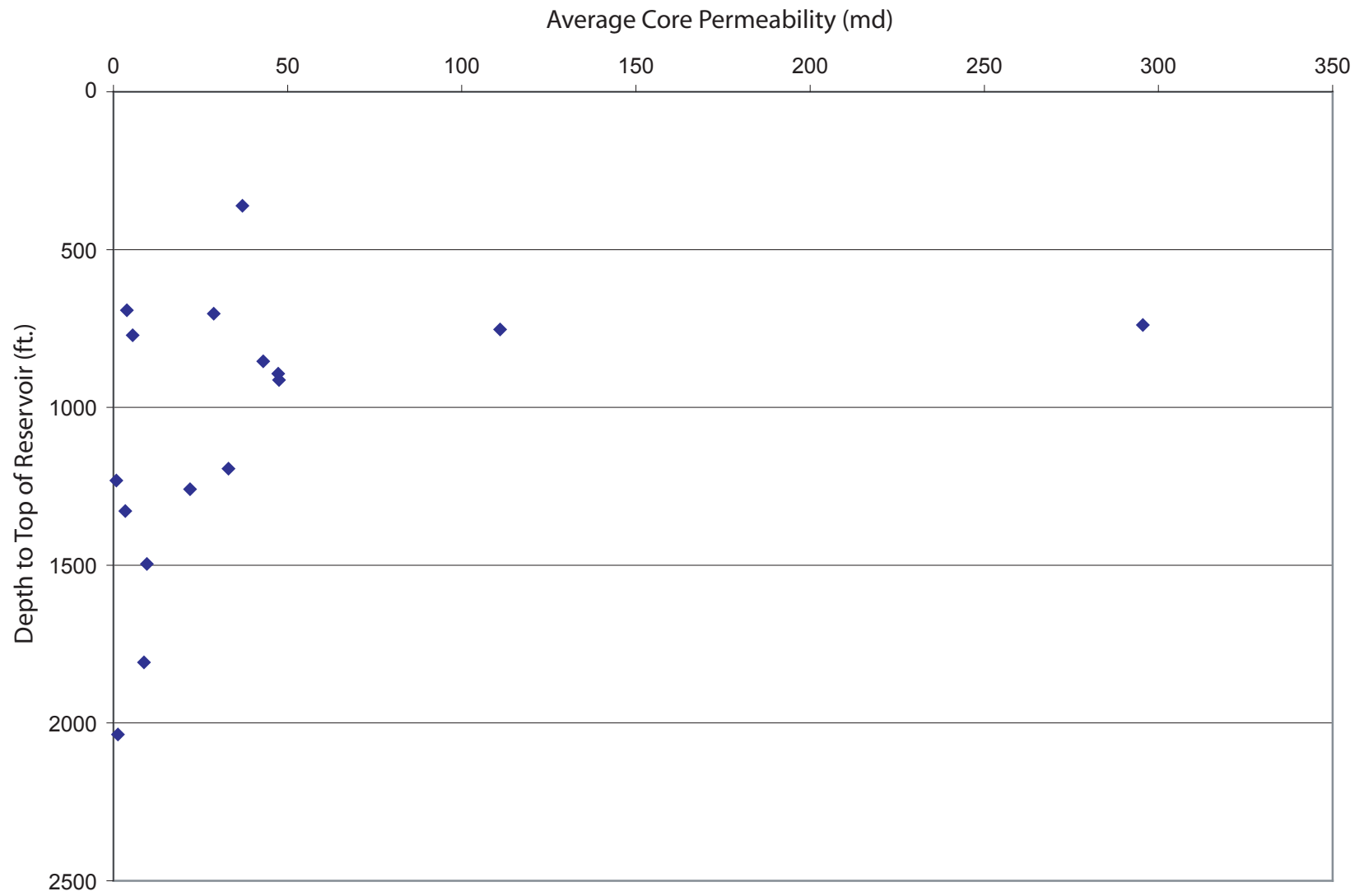
Figure 45. Graph of Berea Sandstone average core permeability vs. depth to top of reservoir (data from Table 11).
