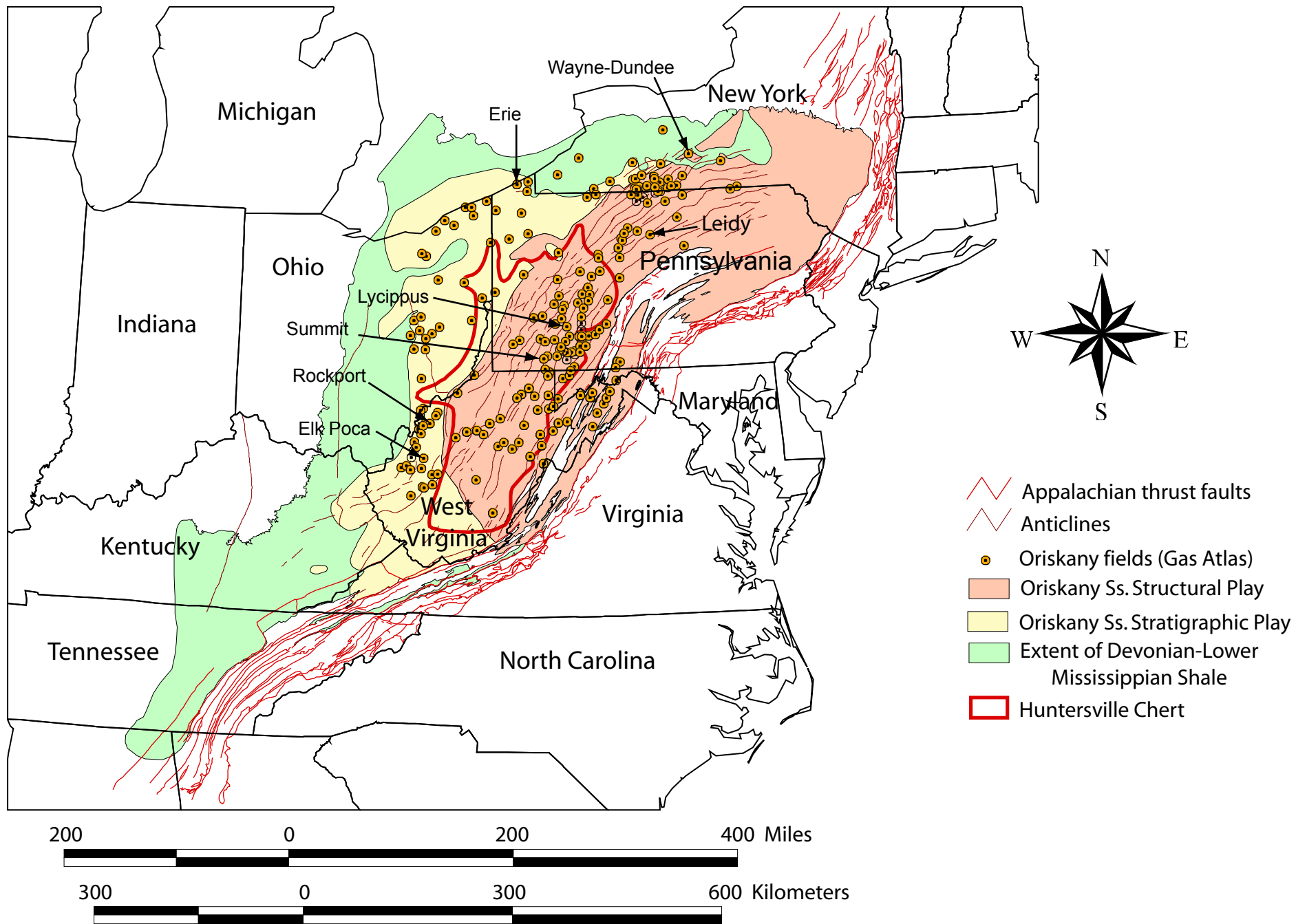
Figure 48. Oriskany Sandstone Structural and Stratigraphic AUs, with gas fields (data from Roen and Walker, 1996).
