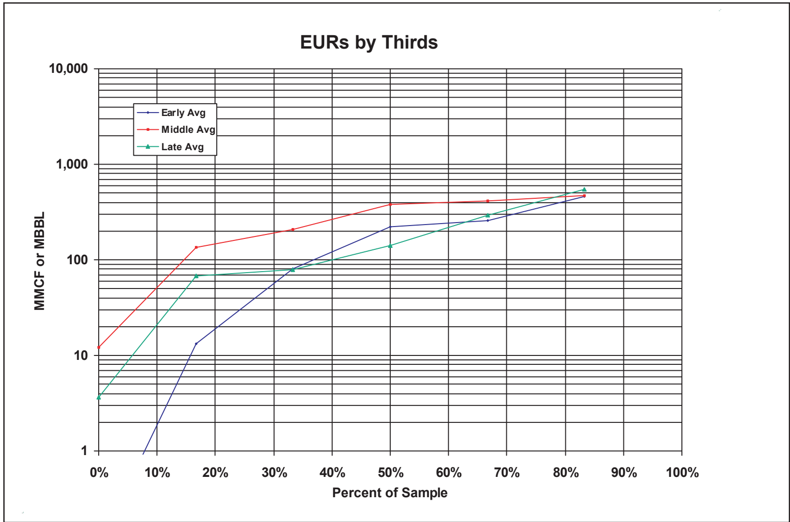
Figure 51. Preliminary distribution of Estimated Ultimate Recovery values (EUR) per well for the Oriskany Sandstone-Stratigraphic AU (thirds); MMCF is million cubic feet, MBBL is thousands of barrels of oil (Troy Cook, USGS, unpublished data 2002).
